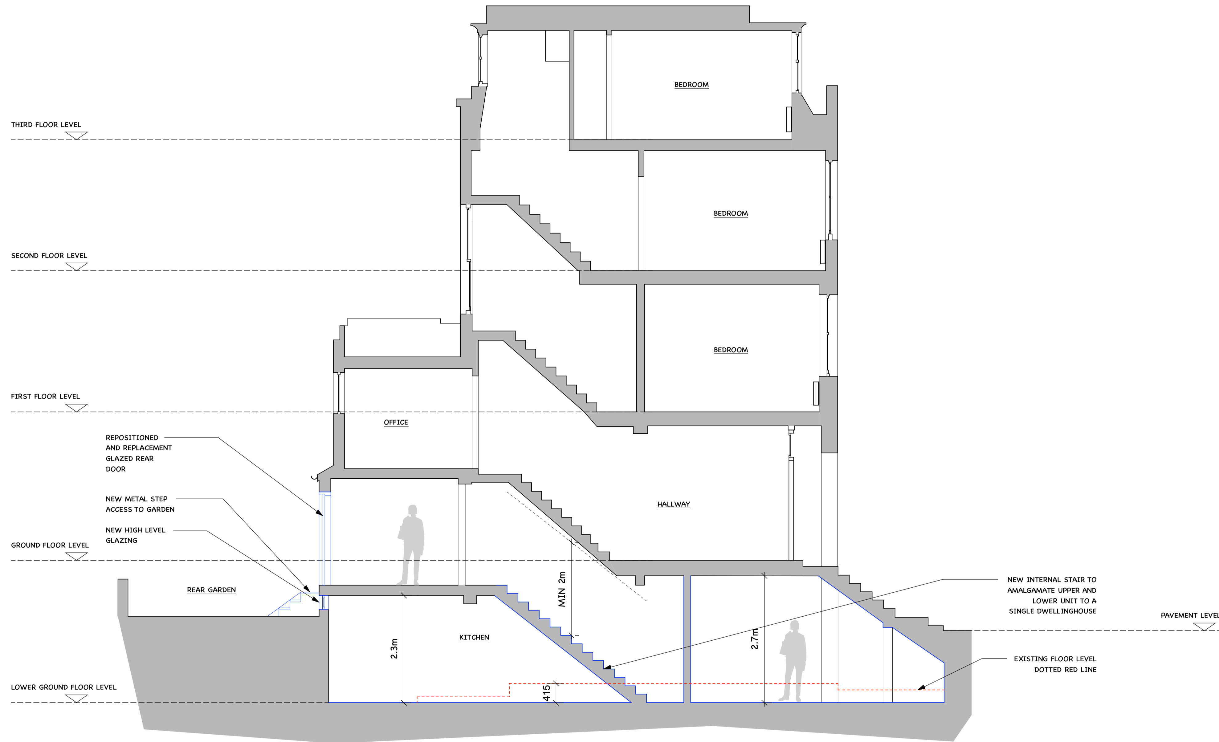
PROPOSED SECTION A-A 1:50 @ A1 / 1:100 @ A3
