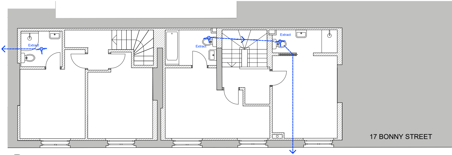
1 FIRST FLOOR MECHANICAL LAYOUT SCALE 1:50 @A1, 1:100 @ A3
