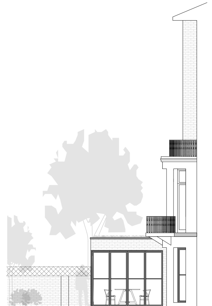
EAST ELEVATION EXTENSION - PROPOSED
