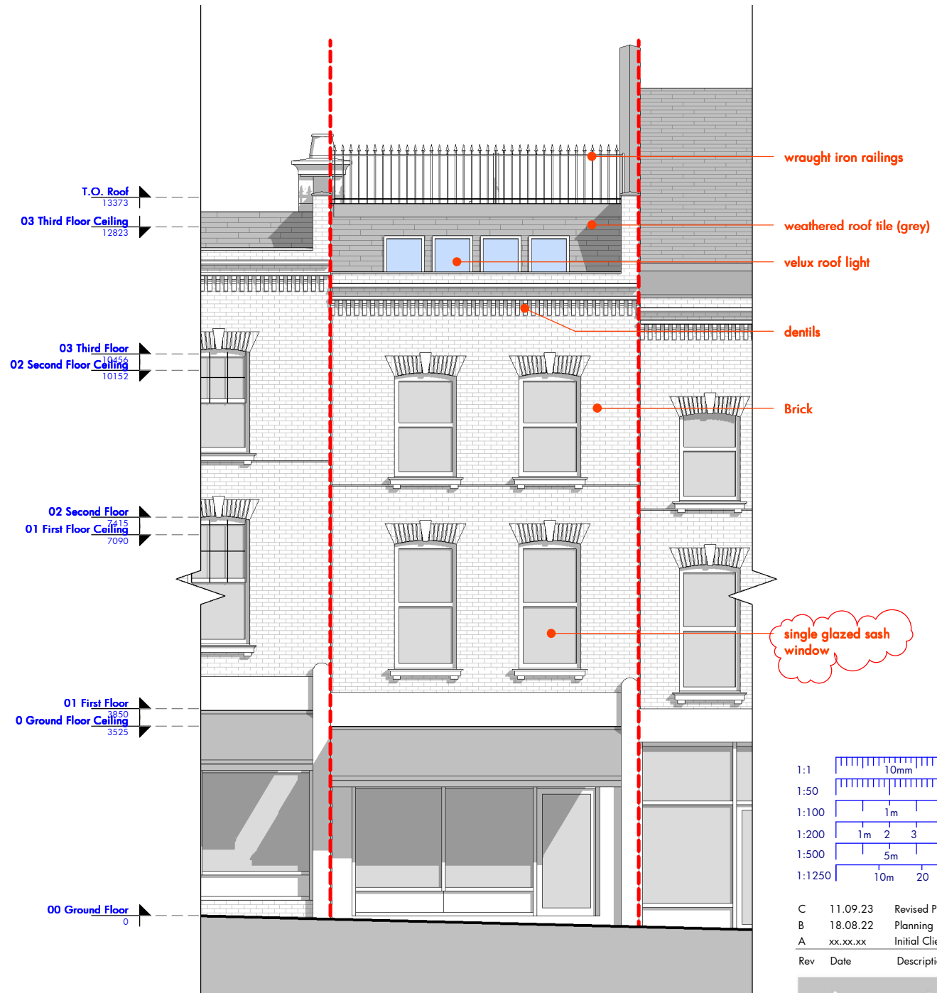
South Elevation (Rosslyn Hill)
