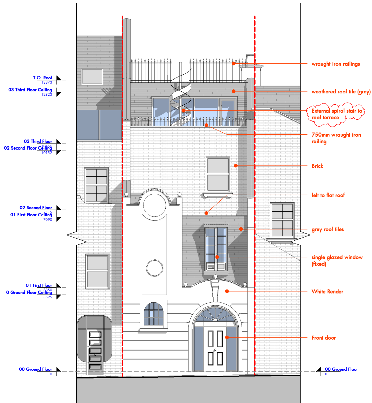
North Elevation (Rosslyn Mews)
