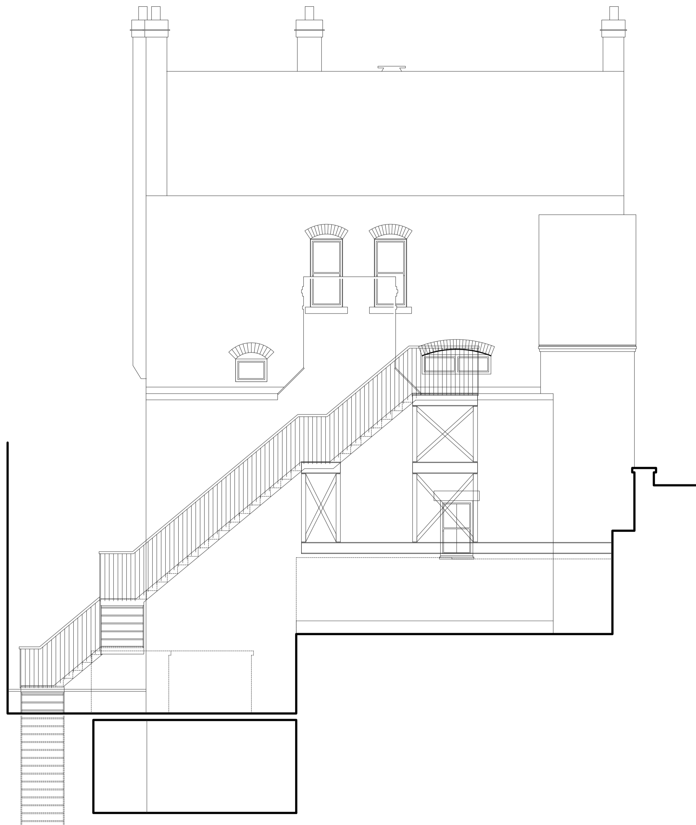
West Elevation
