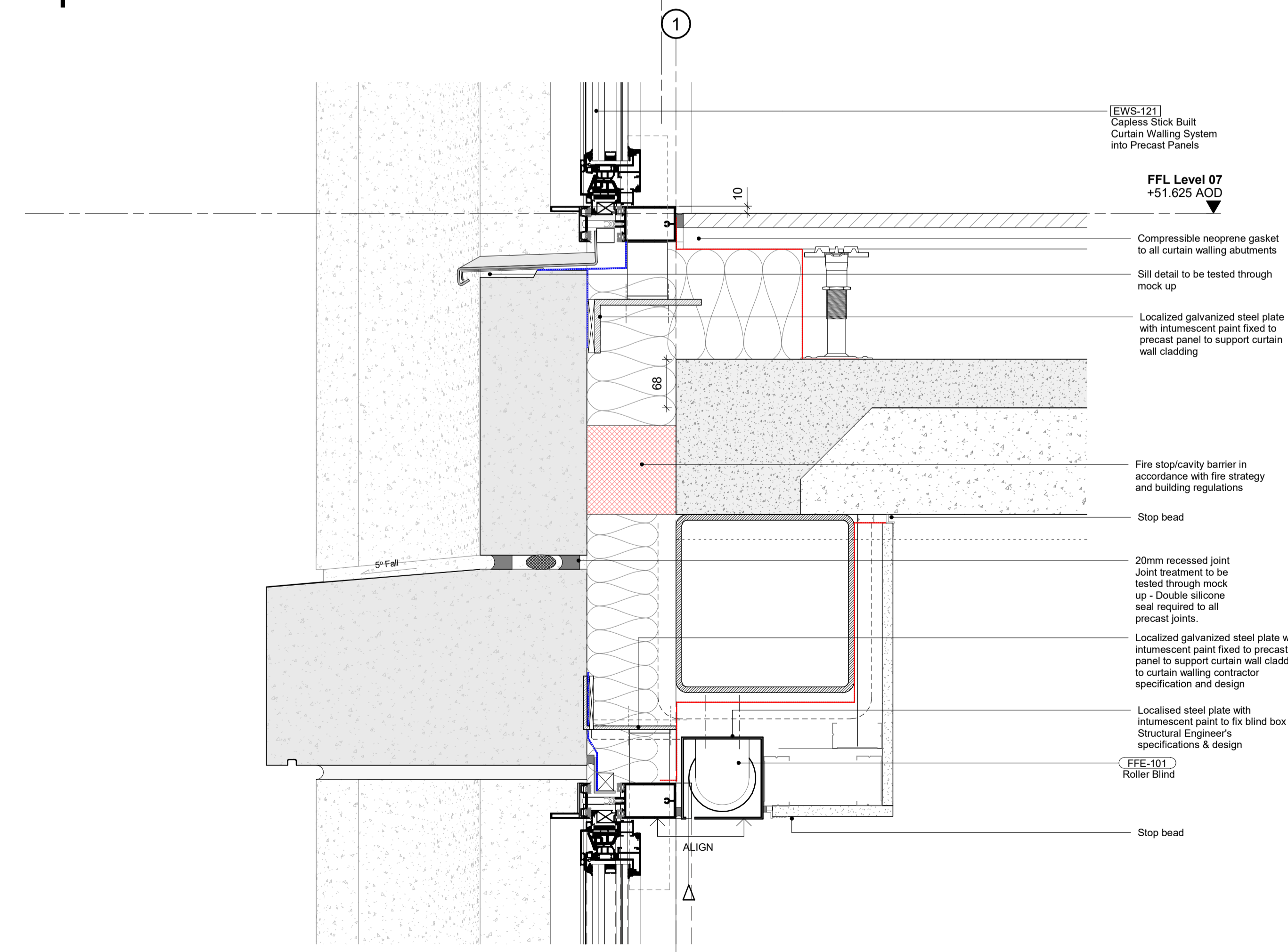
3 Facade Type EWS-821 - Typical Bay Section - At Opening Vent
