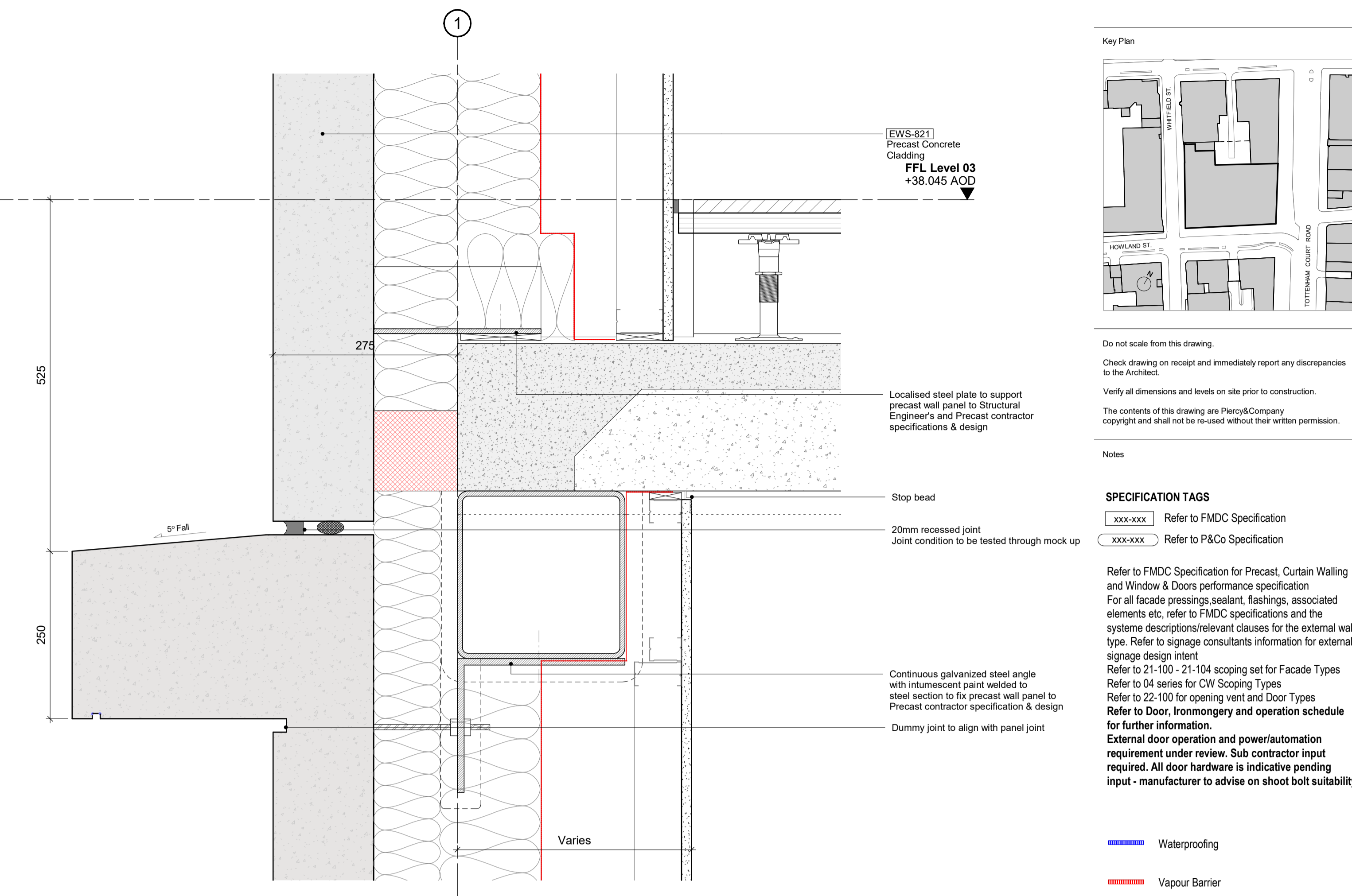
2 Facade Type EWS-821 - Typical Bay Section - At Precast
