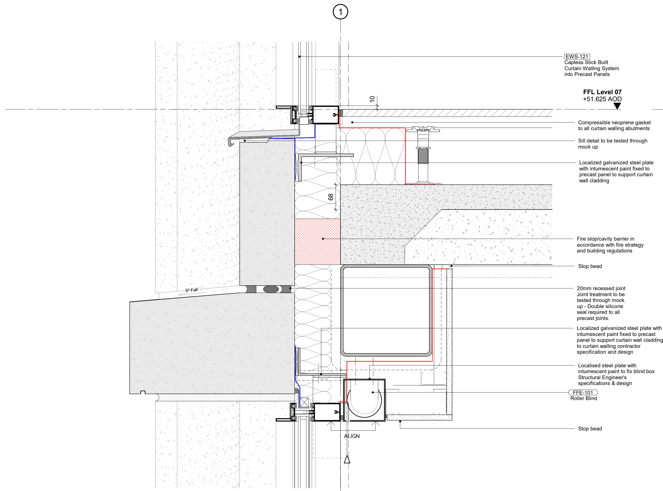
1 Facade Type EWS-821 - Typical Bay Section - At Glazing
