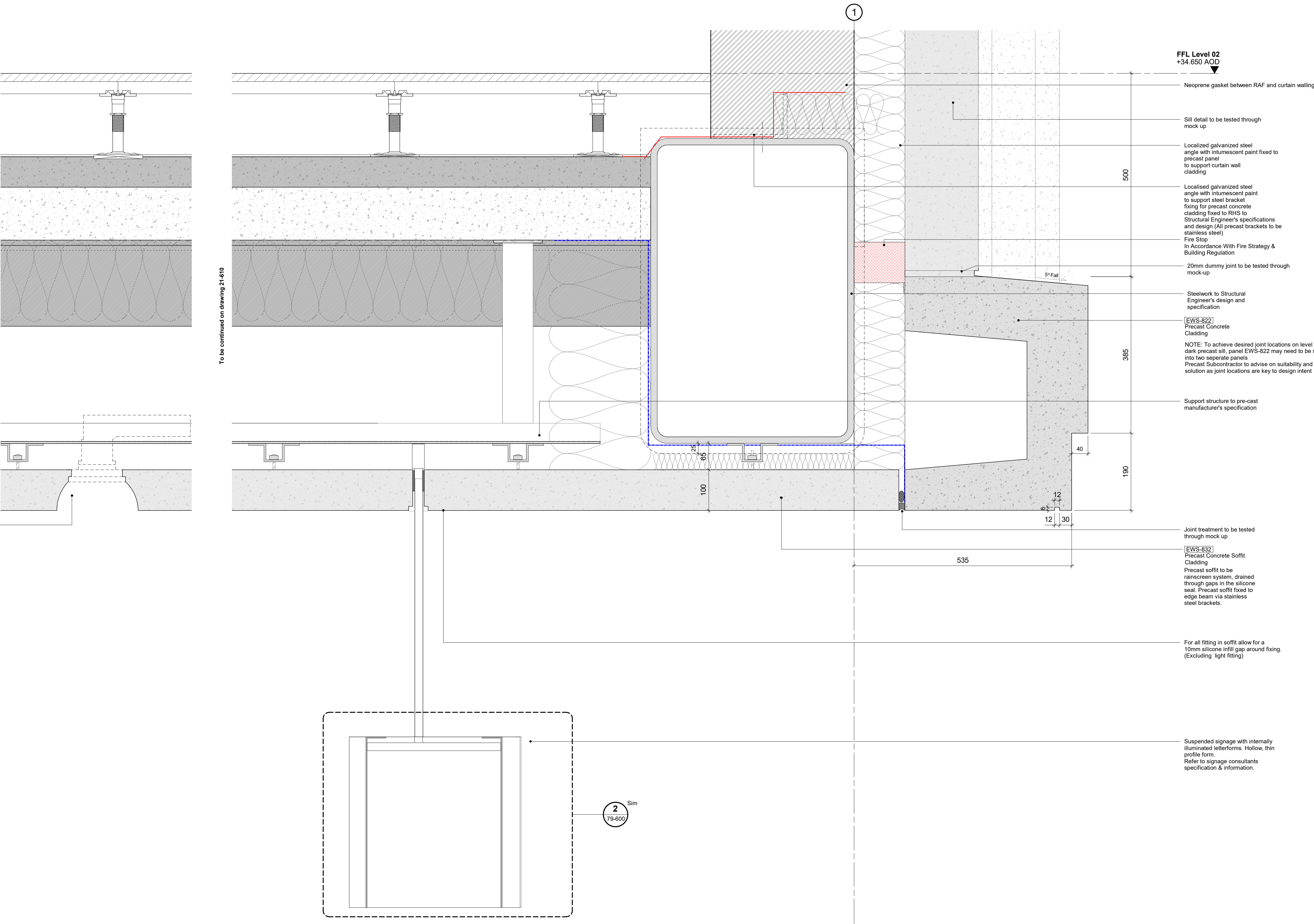
1 Howland St Ground Floor Facade - Curtain Wall Soffit & Sill - Section
