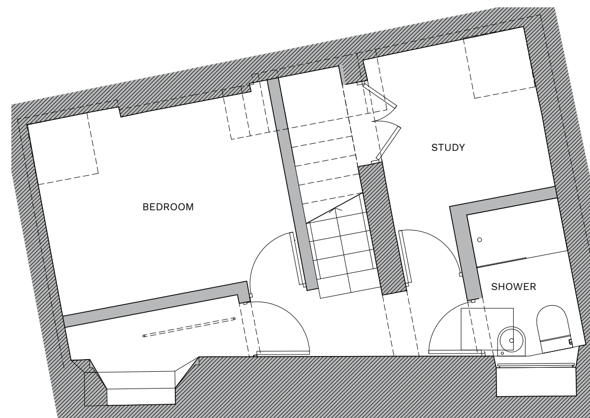
3 PROPOSED LOWER PLAN 1:50 / A3
