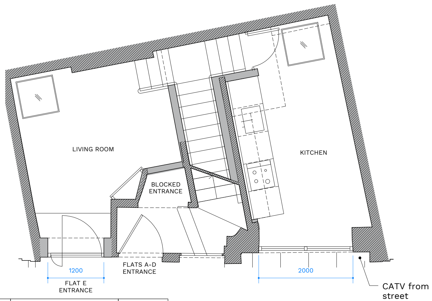
2 PROPOSED GROUND PLAN 1:50 / A2
