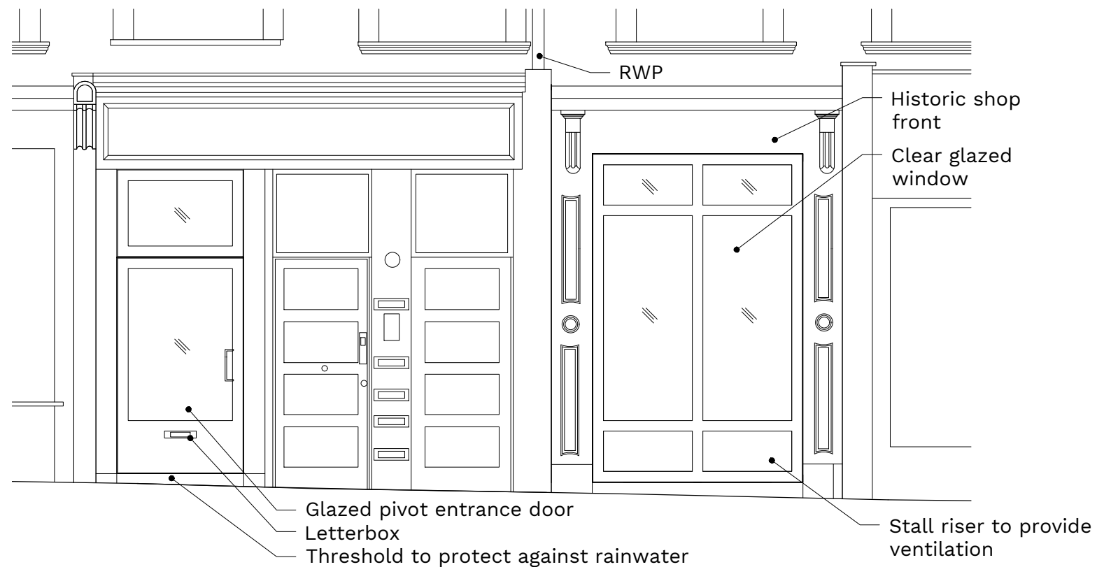
1 PROPOSED ELEVATION 1:50 / A3
