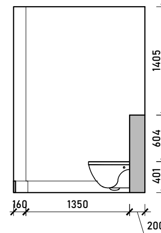
Internal Elevation D
