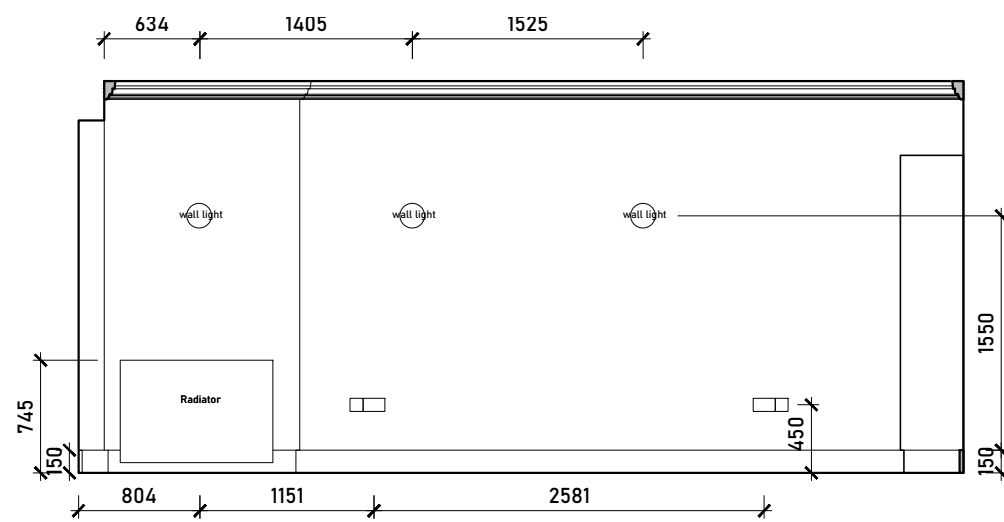
Internal Elevation A
