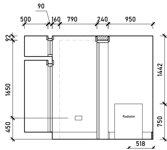
Internal Elevation D
