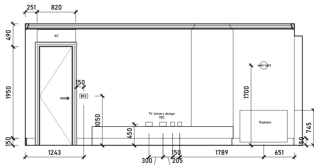
Internal Elevation D
