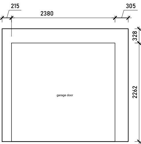
Internal Elevation B
