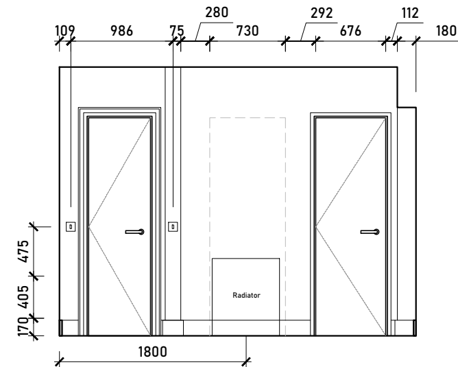
Internal Elevation D
