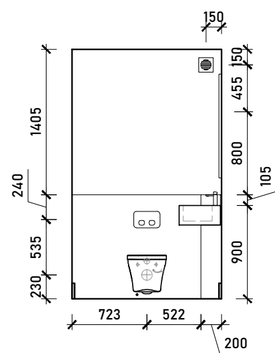
Internal Elevation C
