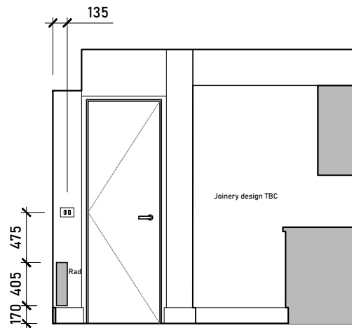
Internal Elevation A
