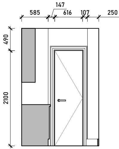
Internal Elevation A
