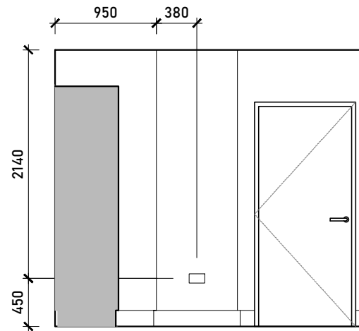
Internal Elevation C
