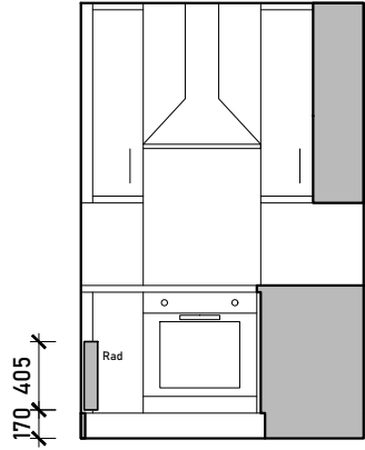
Internal Elevation C
