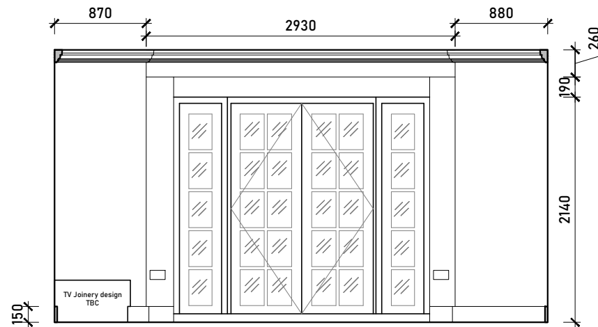
Internal Elevation A
