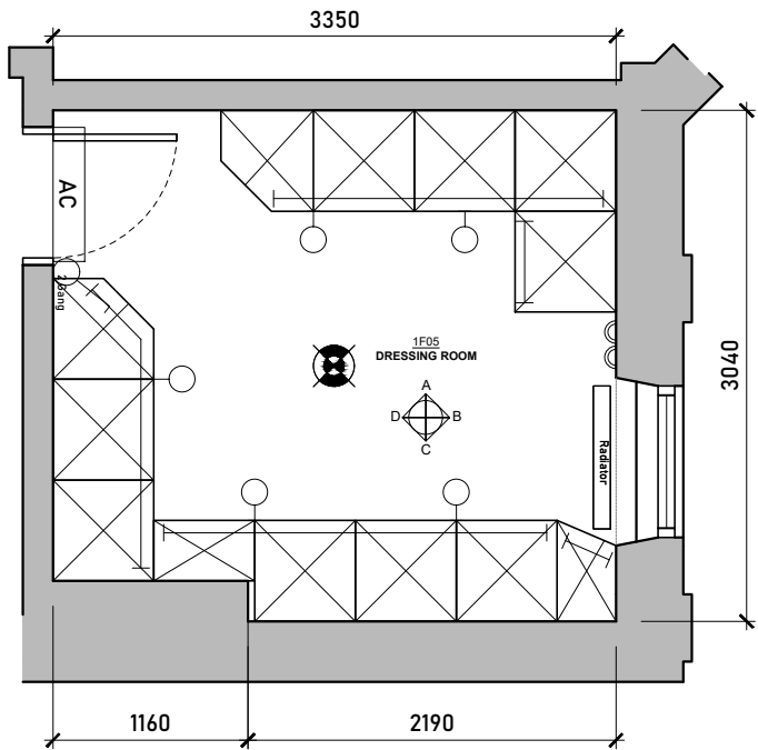
Proposed Dressing Room Floorplan Scale 1:50 @ A3
