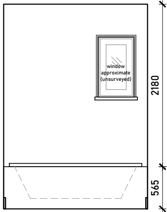
Internal Elevation C
