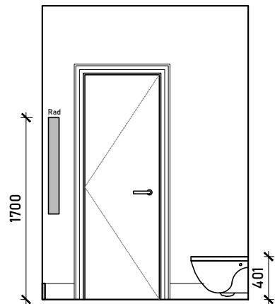
Internal Elevation A
