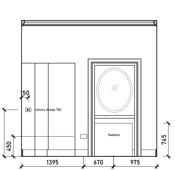
Internal Elevation B
