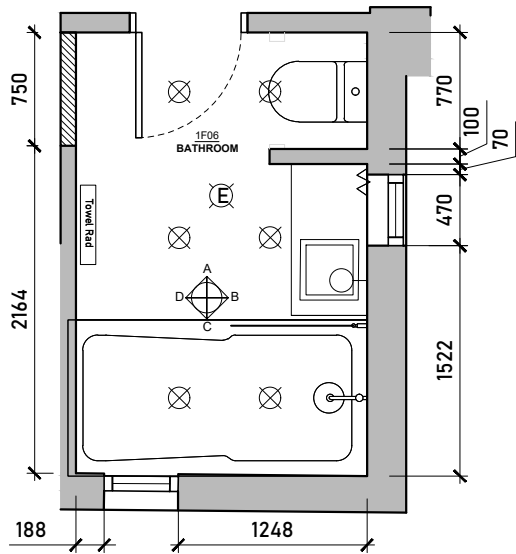
Proposed Bathroom Floorplan Scale 1:50 @ A3
