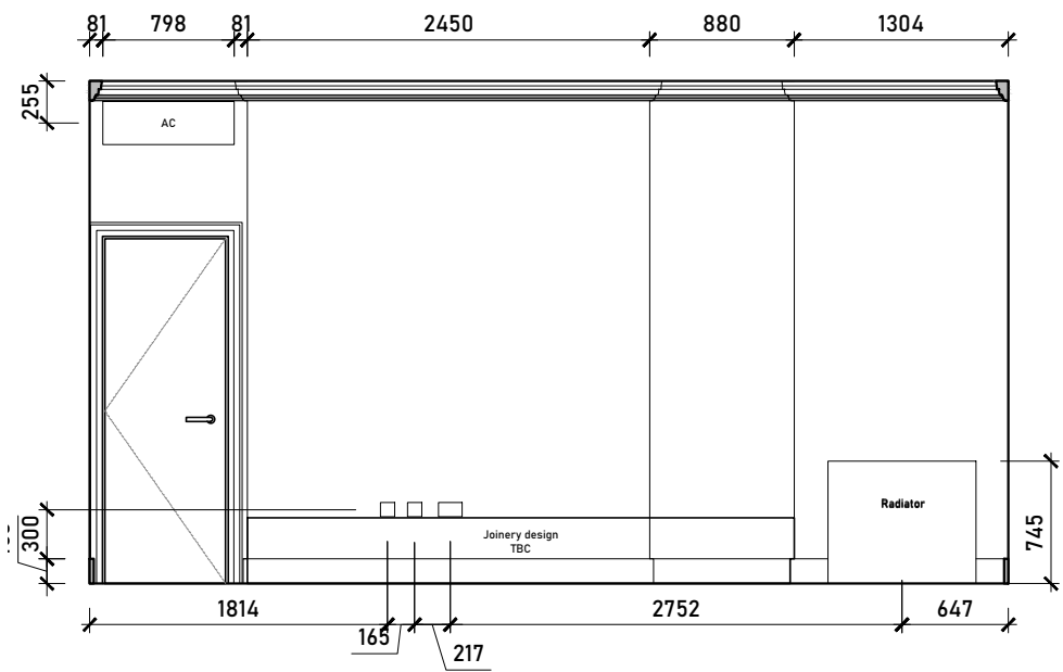
Internal Elevation C
