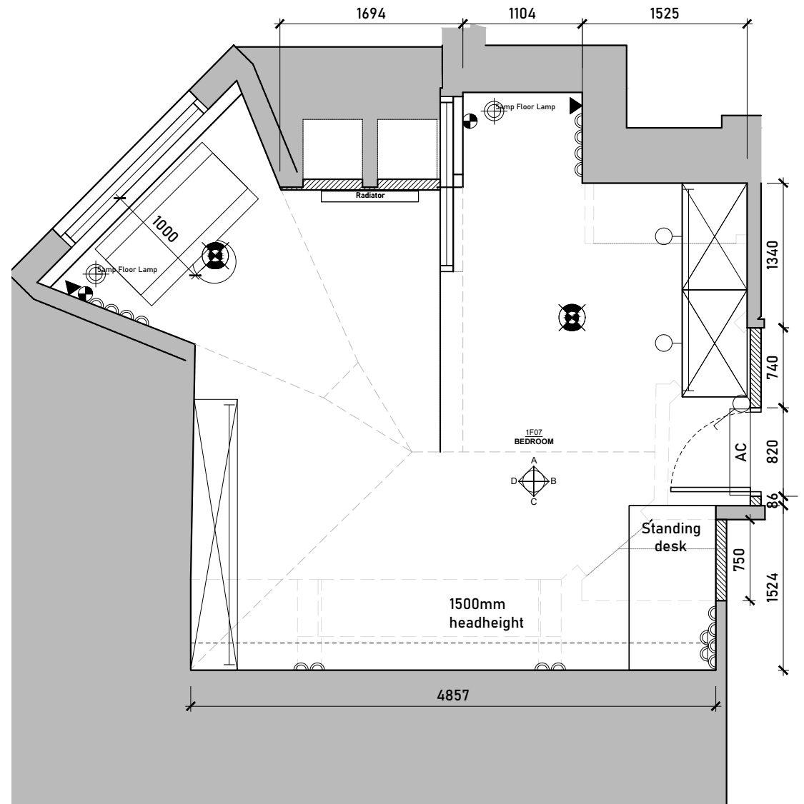
Proposed Bedroom Floorplan Scale 1:50 @ A3
