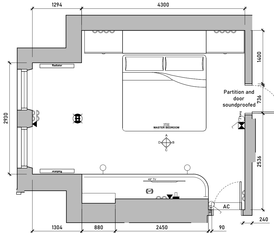
Proposed Master Bedroom Floorplan Scale 1:50 @ A3
