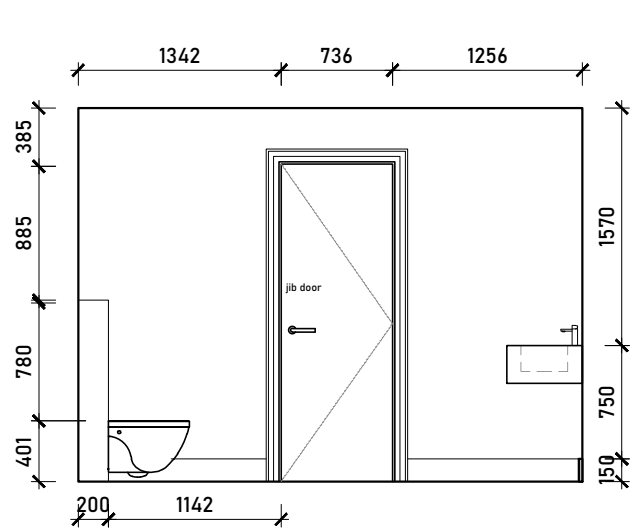
Internal Elevation B
