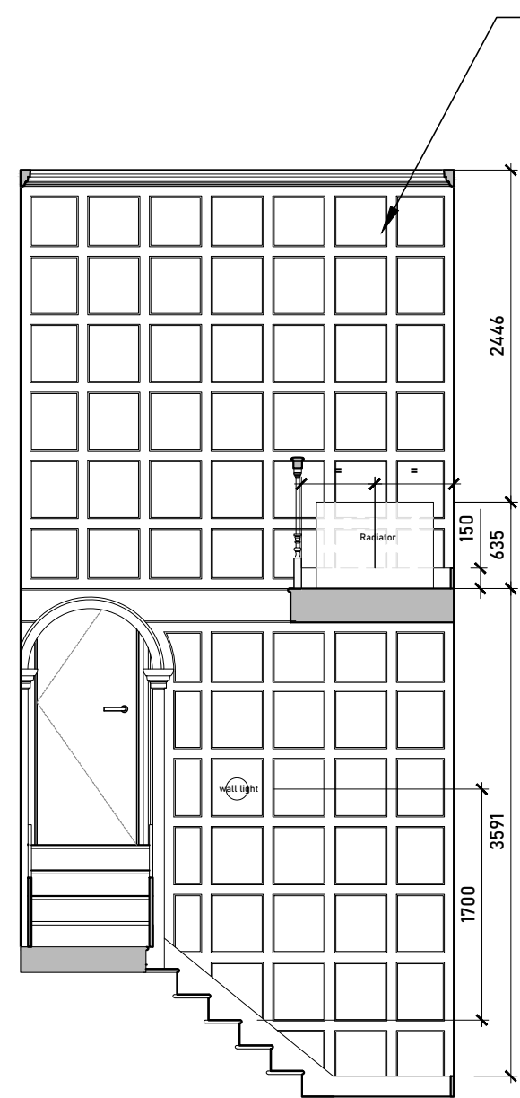
Internal Elevation D_02
