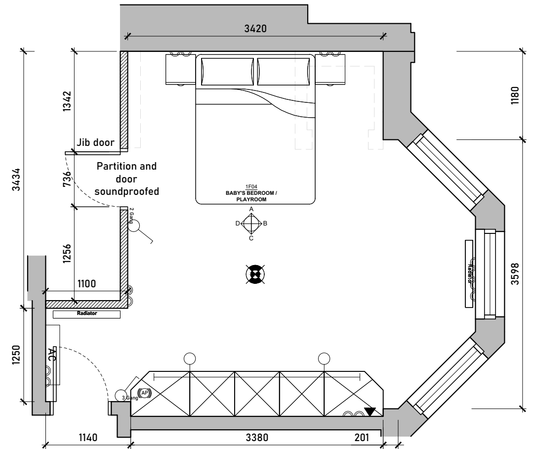
Proposed Playroom Floorplan Scale 1:50 @ A3
