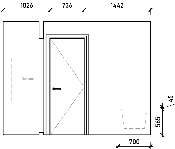
Internal Elevation D
