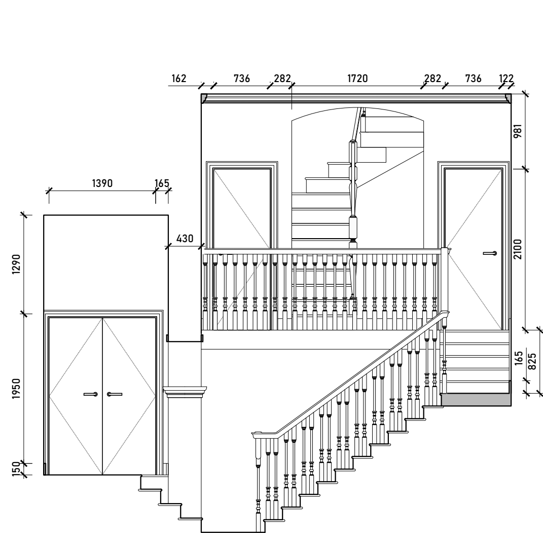
Internal Elevation A
