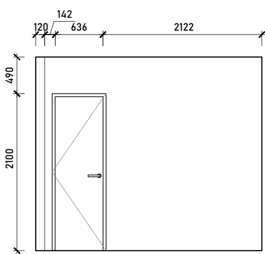
Internal Elevation B
