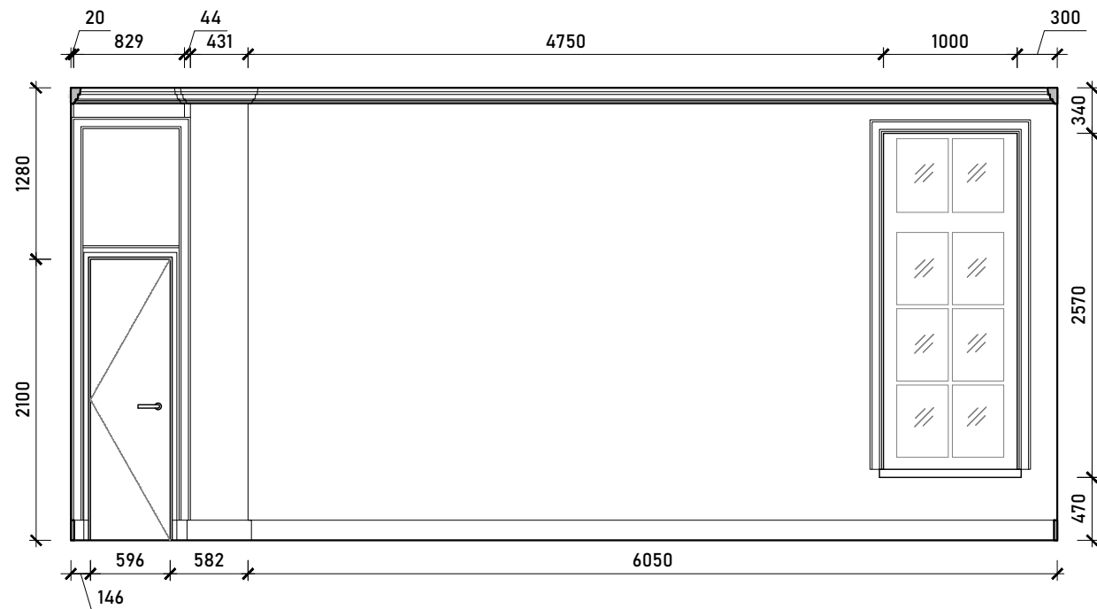
Internal Elevation A
