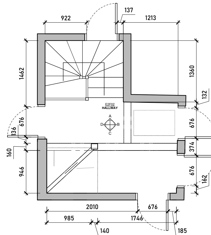
Existing Hallway Floorplan Scale 1:50 @ A3
