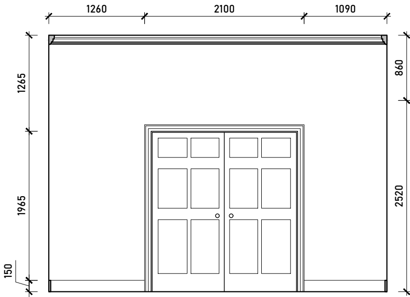
Internal Elevation B
