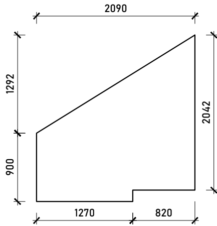
Internal Elevation C
