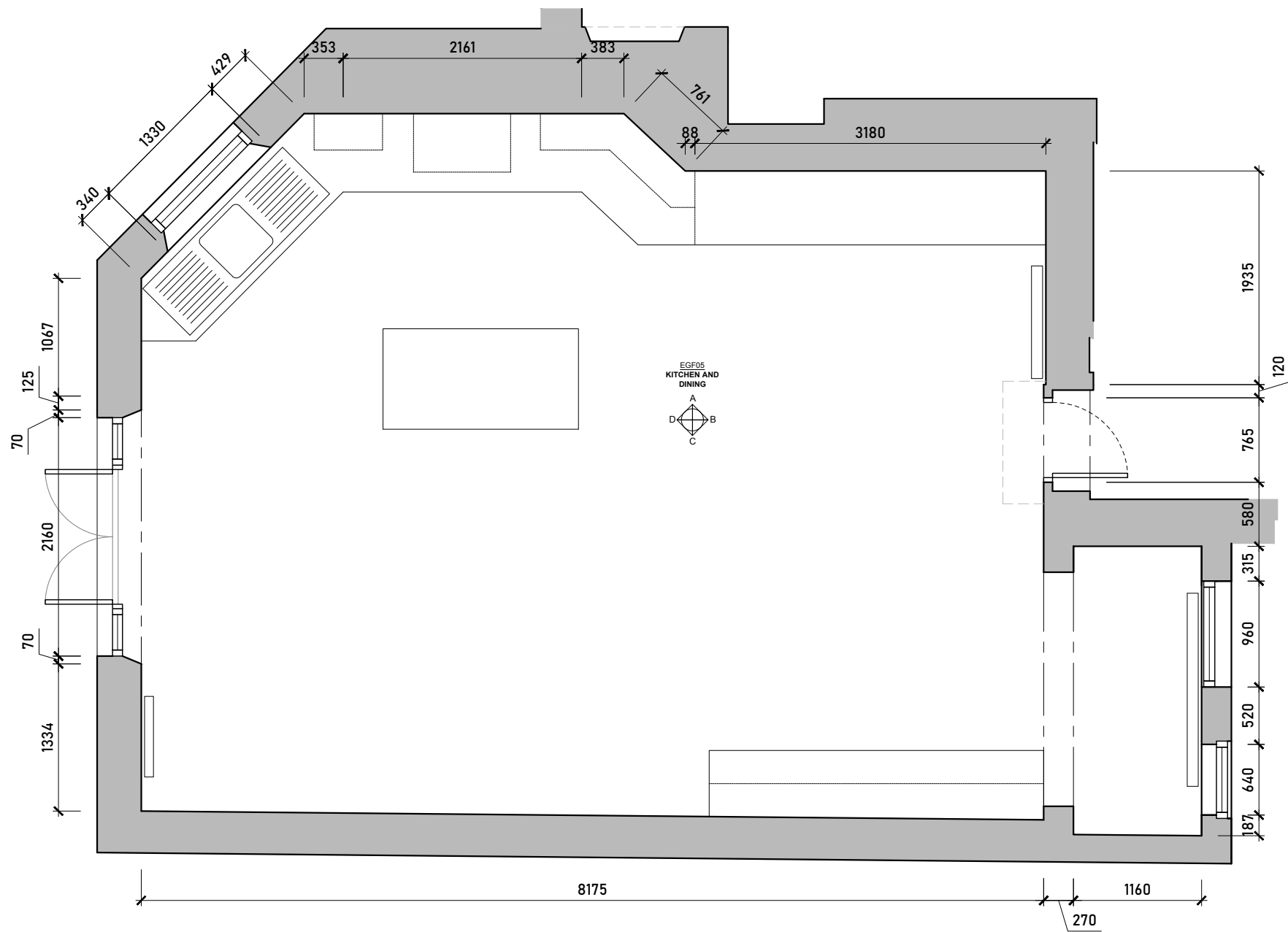
Existing Kitchen Floorplan Scale 1:50 @ A3
