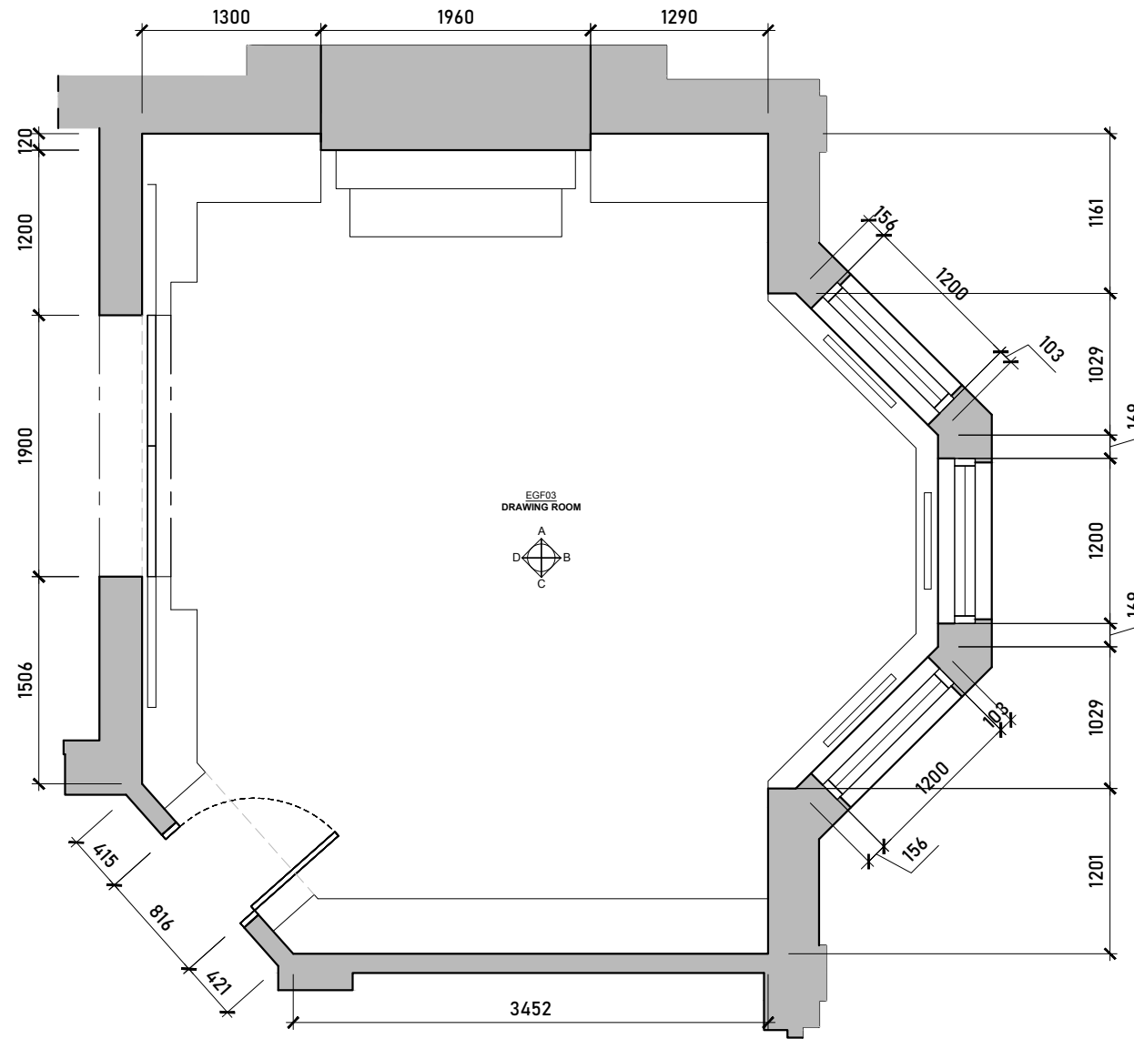
Existing Drawing Room Floorplan Scale 1:50 @ A3
