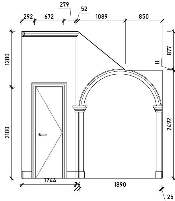
Internal Elevation B
