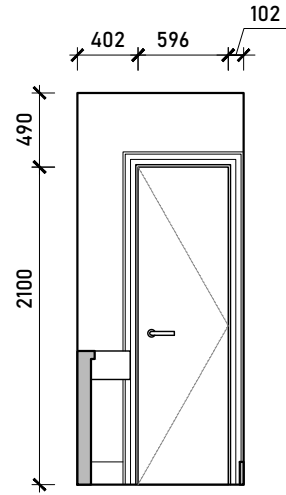
Internal Elevation B
