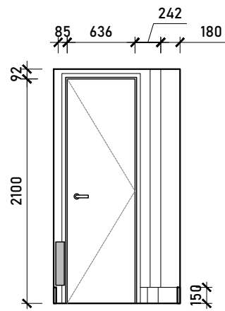
Internal Elevation A
