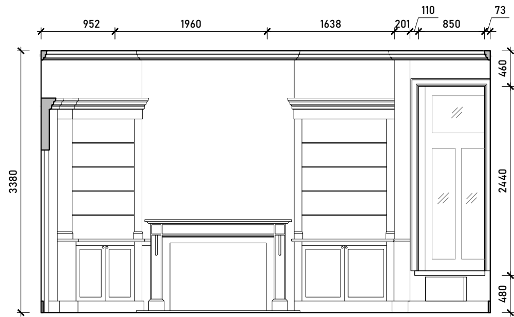
Internal Elevation A
