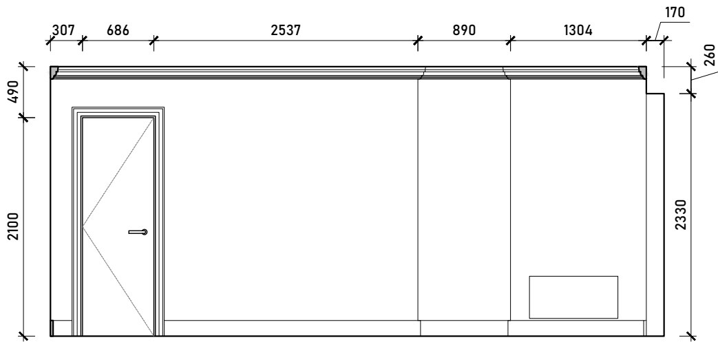
Internal Elevation C
