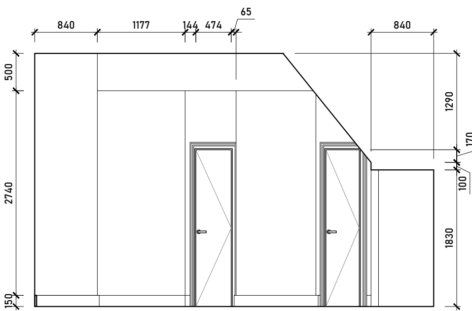
Internal Elevation A
