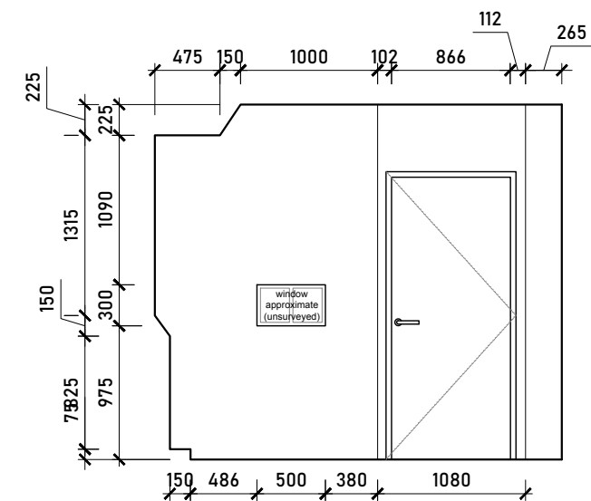
Internal Elevation A
