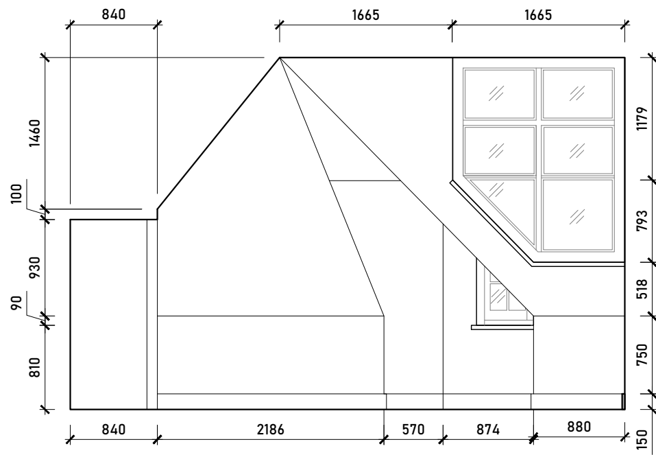
Internal Elevation A
