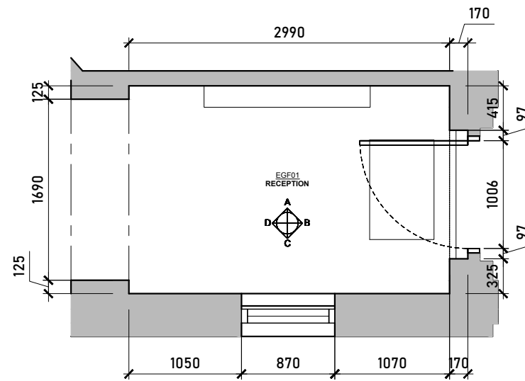
Existing Reception Floorplan Scale 1:50 @ A3
