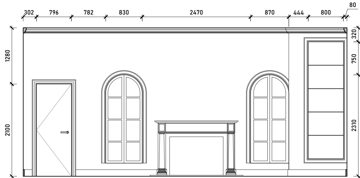
Internal Elevation A
