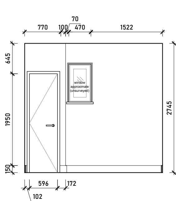
Internal Elevation B
