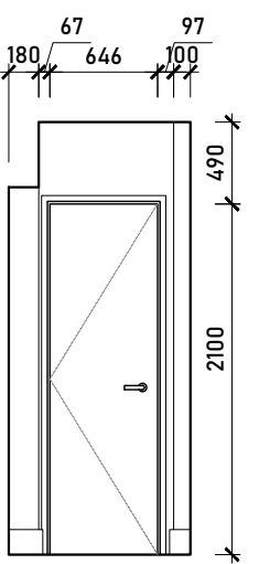
Internal Elevation B
