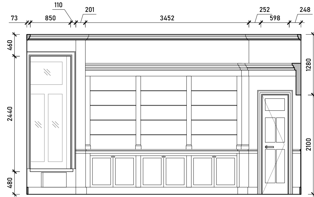
Internal Elevation C
