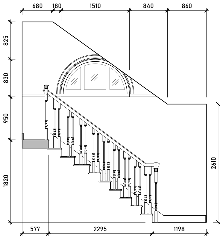
Internal Elevation C
