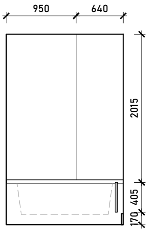
Internal Elevation C
