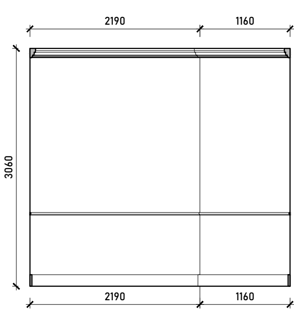
Internal Elevation C
