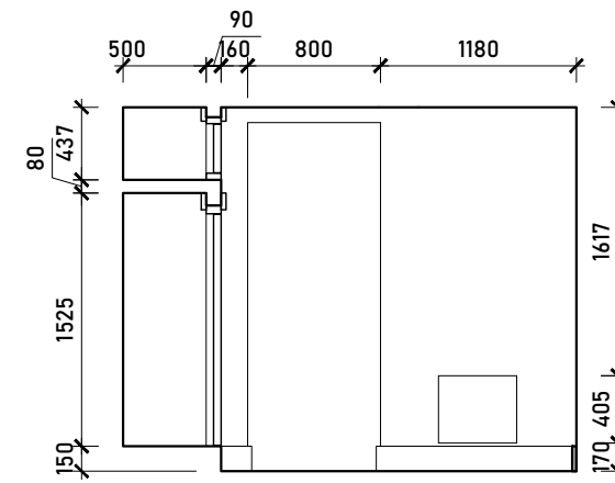
Internal Elevation D
