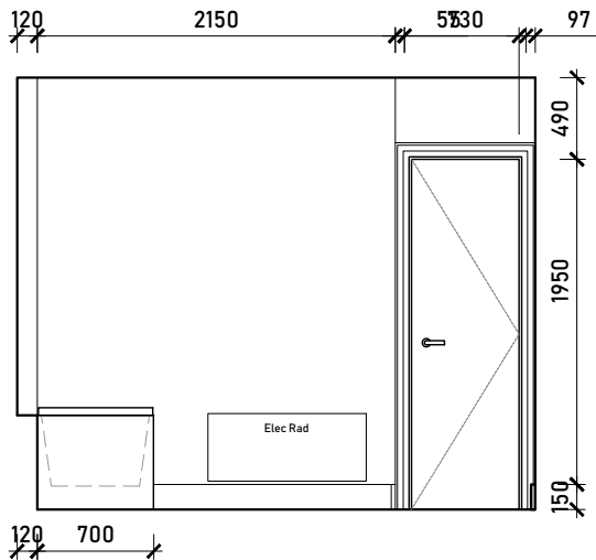
Internal Elevation D
