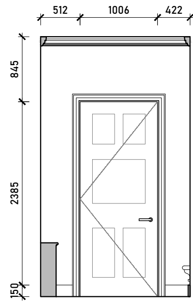
Internal Elevation B
