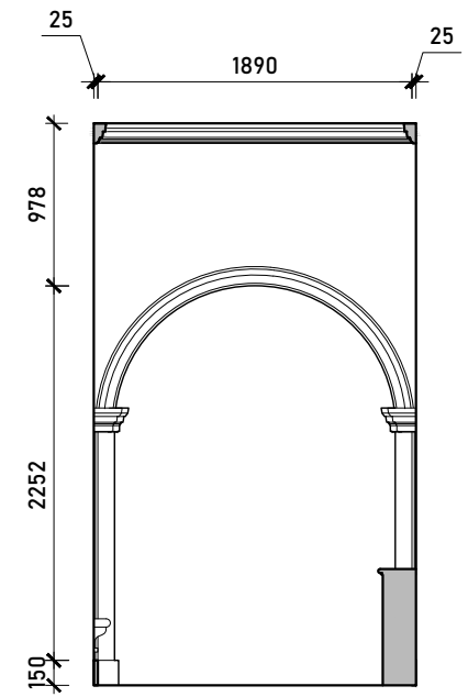
Internal Elevation D
