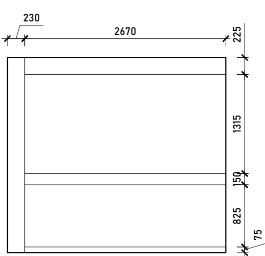
Internal Elevation D
