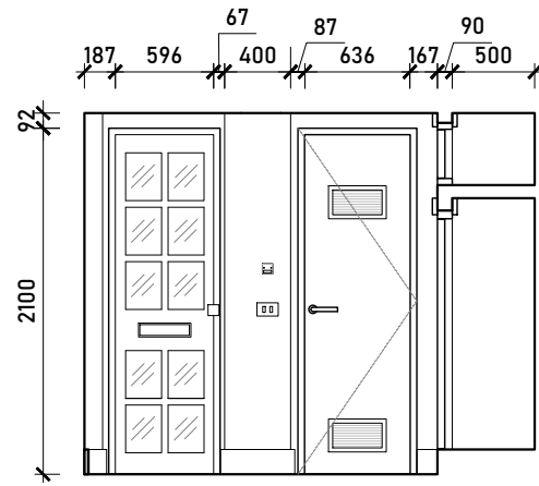
Internal Elevation B
