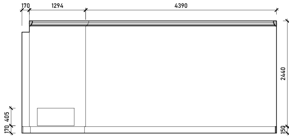
Internal Elevation A
