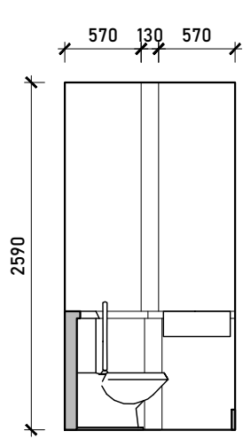
Internal Elevation A
