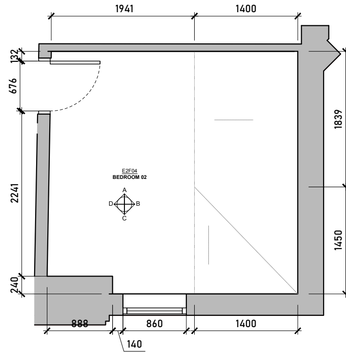
Existing Bedroom Floorplan Scale 1:50 @ A3
