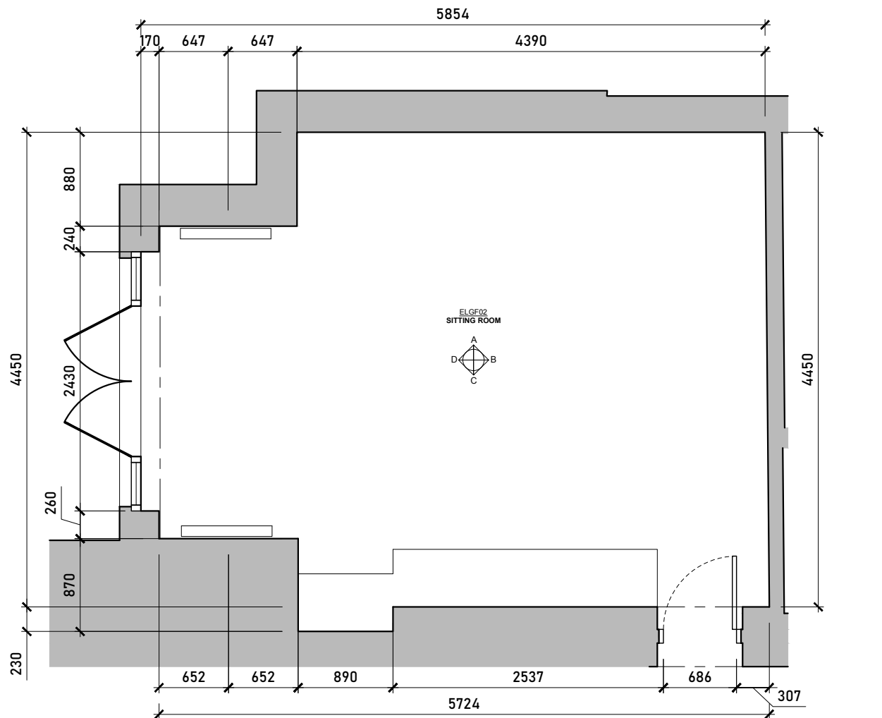
Existing Sitting Room Floorplan Scale 1:50 @ A3
