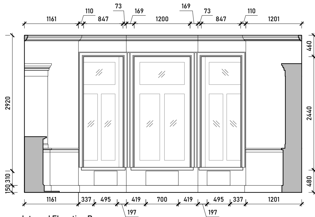
Internal Elevation B
