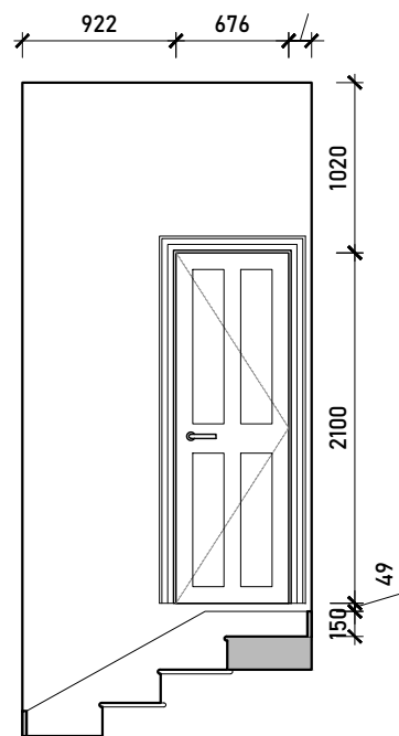
Internal Elevation A
