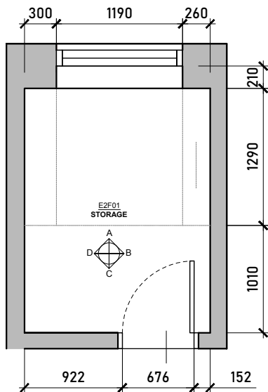
Existing Storage Room Floorplan Scale 1:50 @ A3
