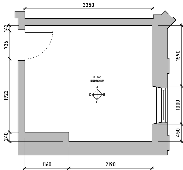
Existing Bedroom Floorplan Scale 1:50 @ A3
