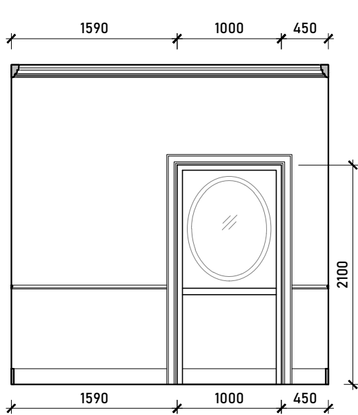
Internal Elevation B
