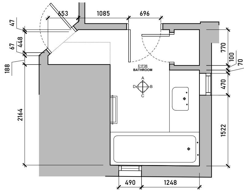
Existing Bathroom Floorplan Scale 1:50 @ A3
