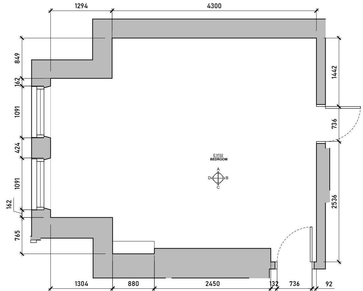
Existing Bedroom Floorplan
