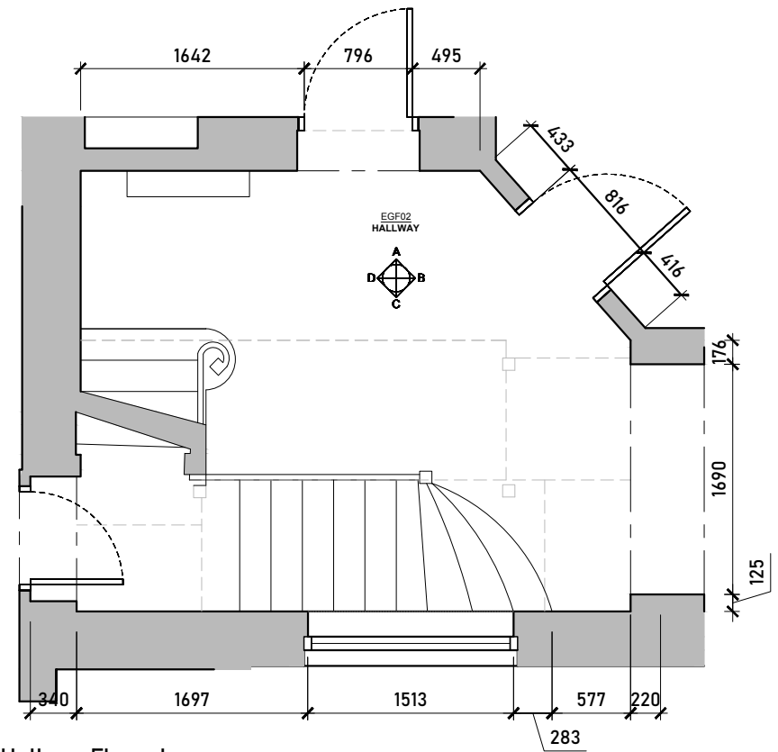
Existing Hallway Floorplan Scale 1:50 @ A3
