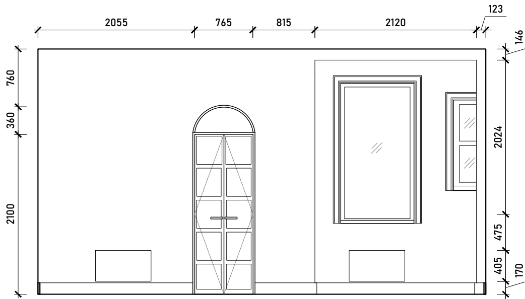
Internal Elevation B
