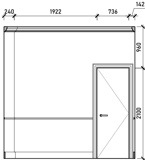
Internal Elevation D
