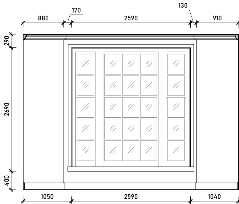
Internal Elevation D
