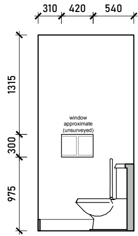
Internal Elevation C
