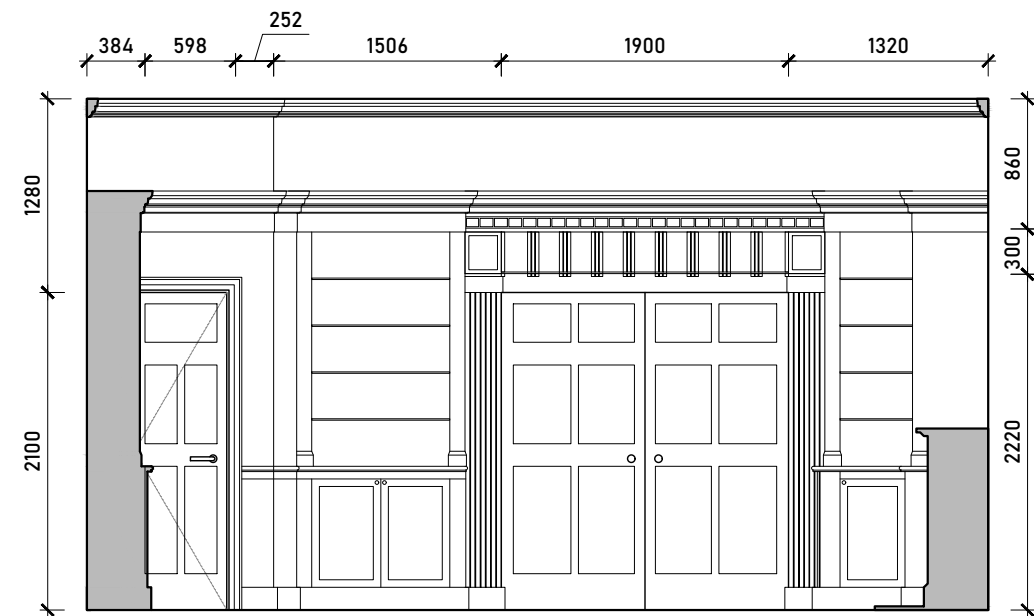
Internal Elevation D
