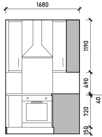
Internal Elevation C
