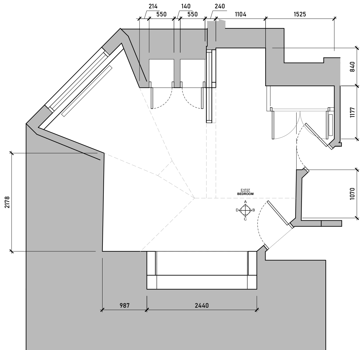
Existing Bedroom Floorplan Scale 1:50 @ A3
