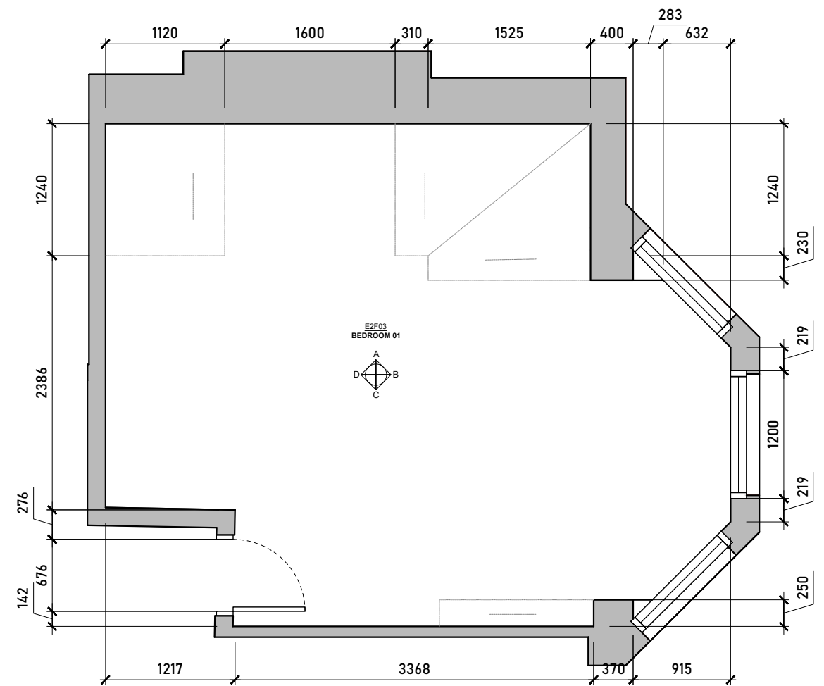
Existing Bedroom Floorplan Scale 1:50 @ A3
