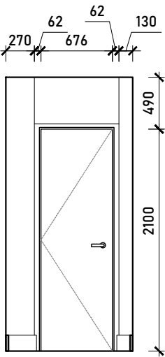
Internal Elevation A
