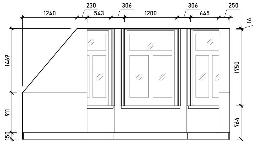
Internal Elevation B
