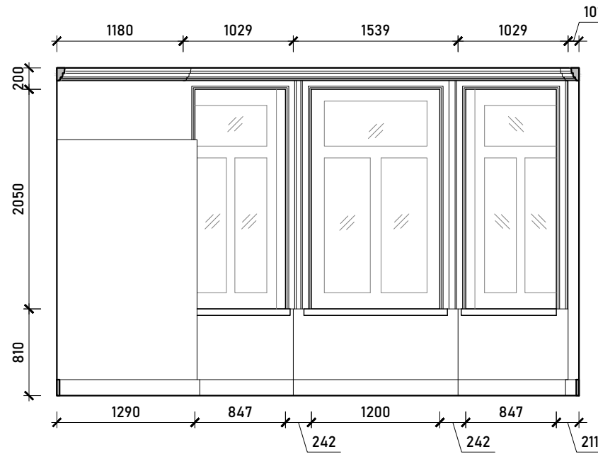
Internal Elevation B
