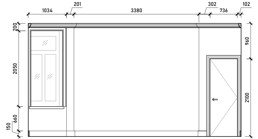
Internal Elevation C
