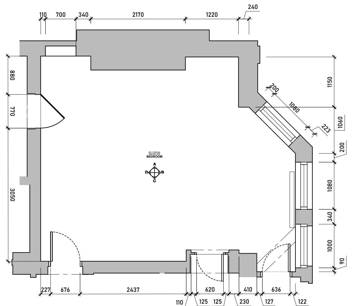
Existing Bedroom Floorplan Scale 1:50 @ A3
