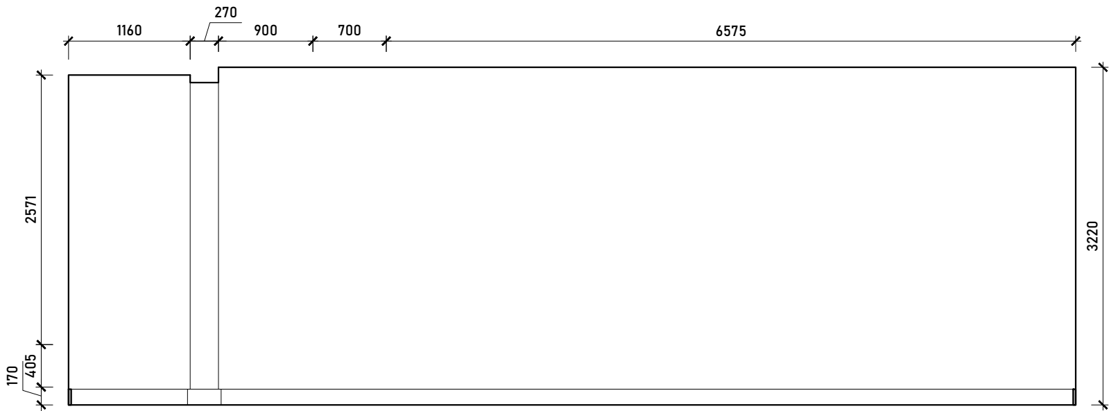
Internal Elevation C
