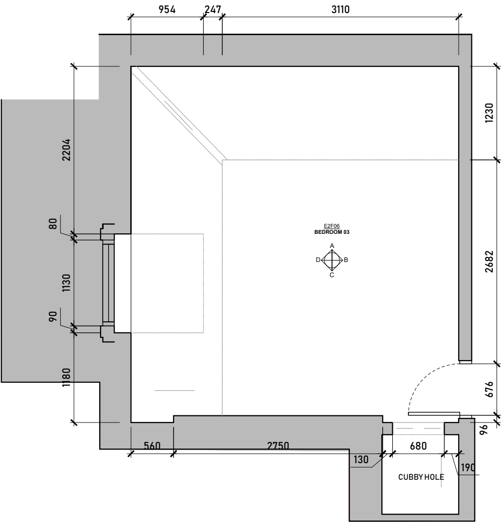
Existing Bedroom Floorplan Scale 1:50 @ A3
