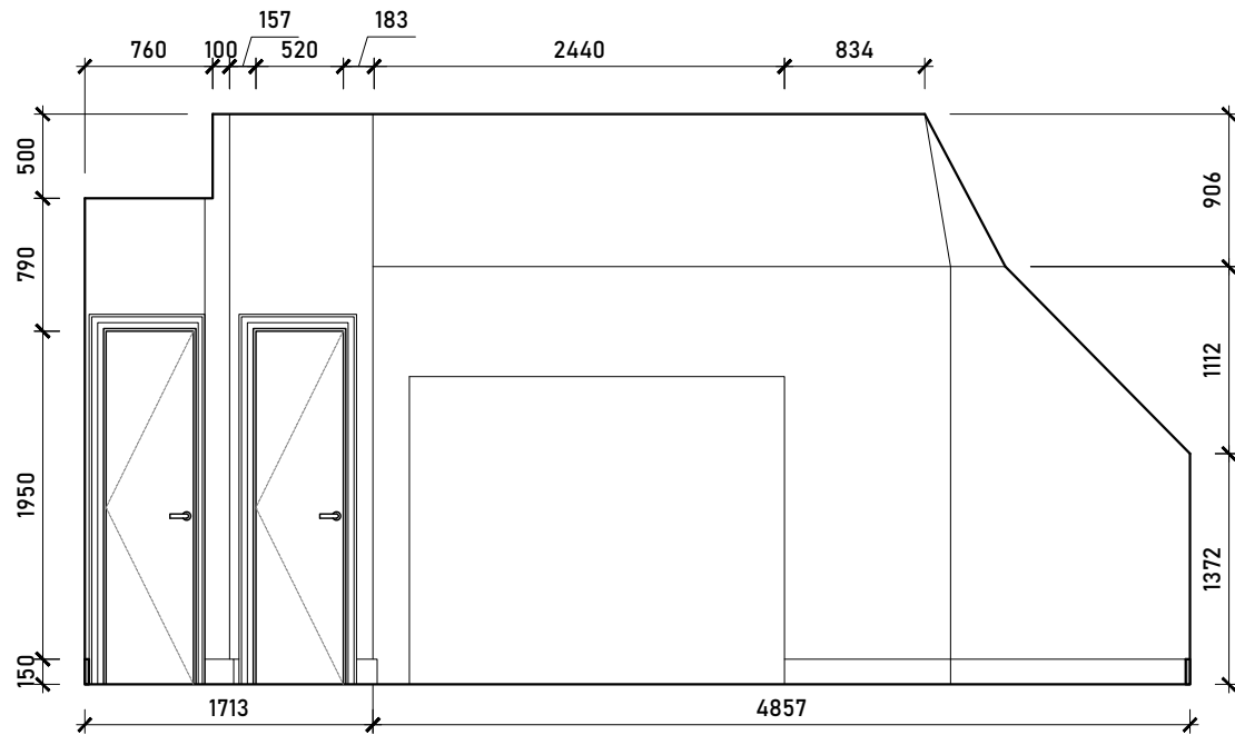
Internal Elevation B
