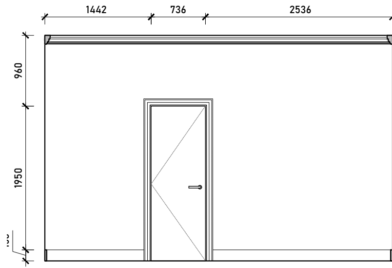
Internal Elevation B
