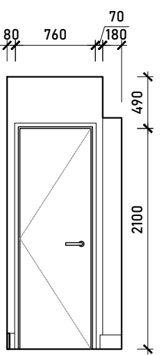
Internal Elevation D
