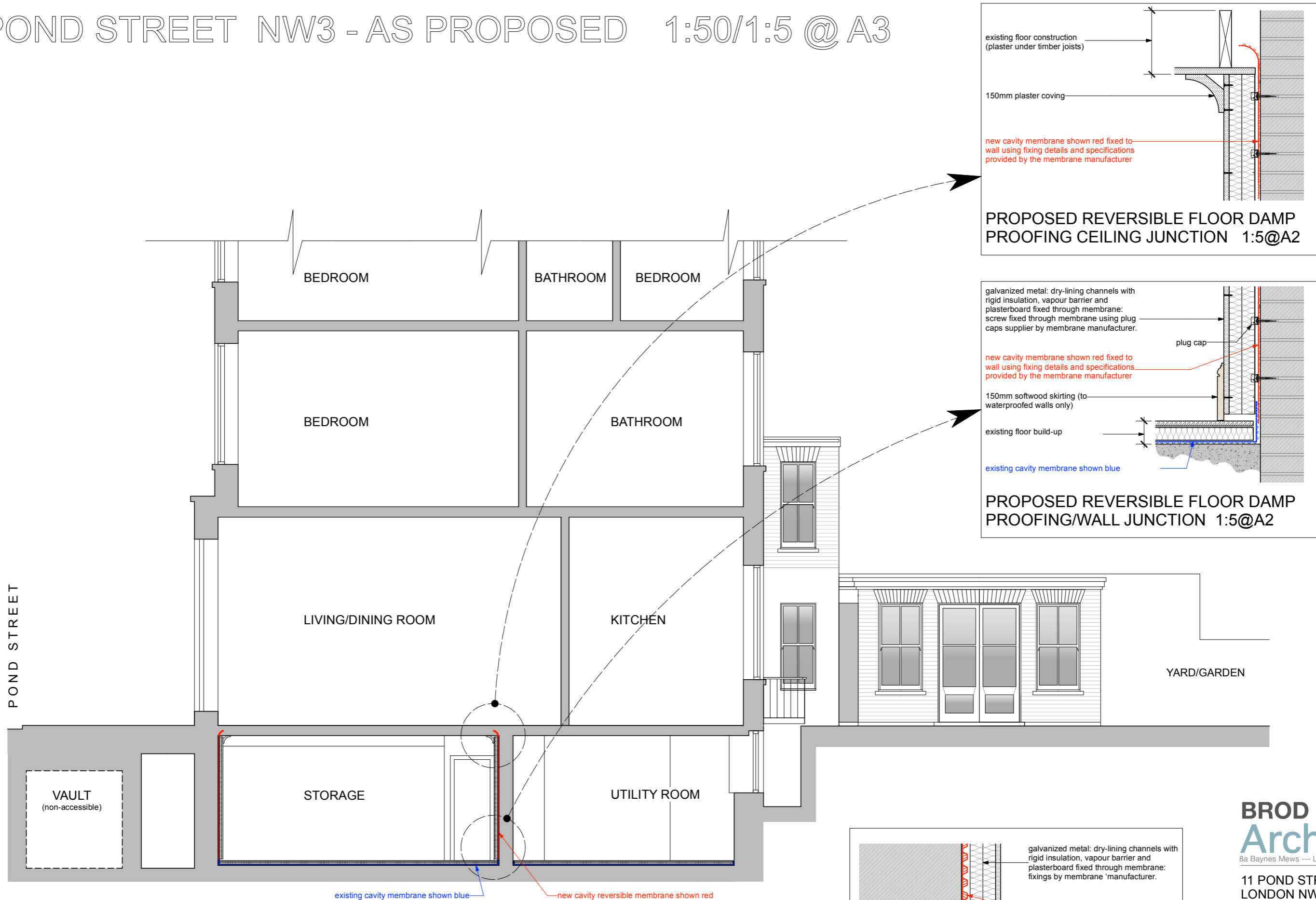
SECTION A-A - PROPOSED
