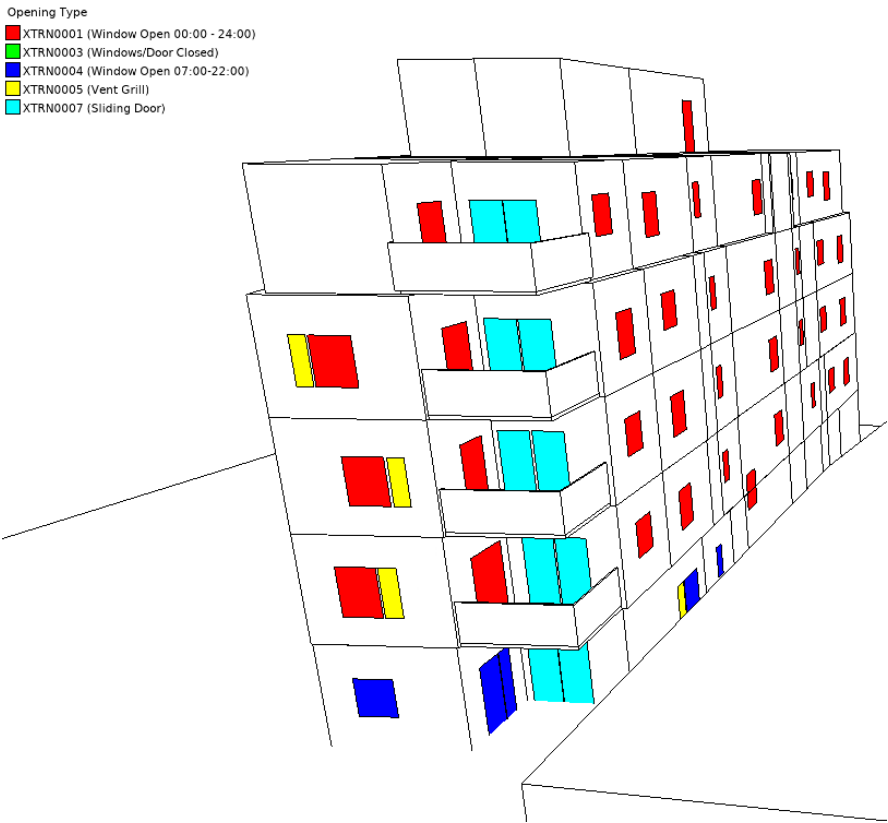
Image 3: Opening type –East Elevation
