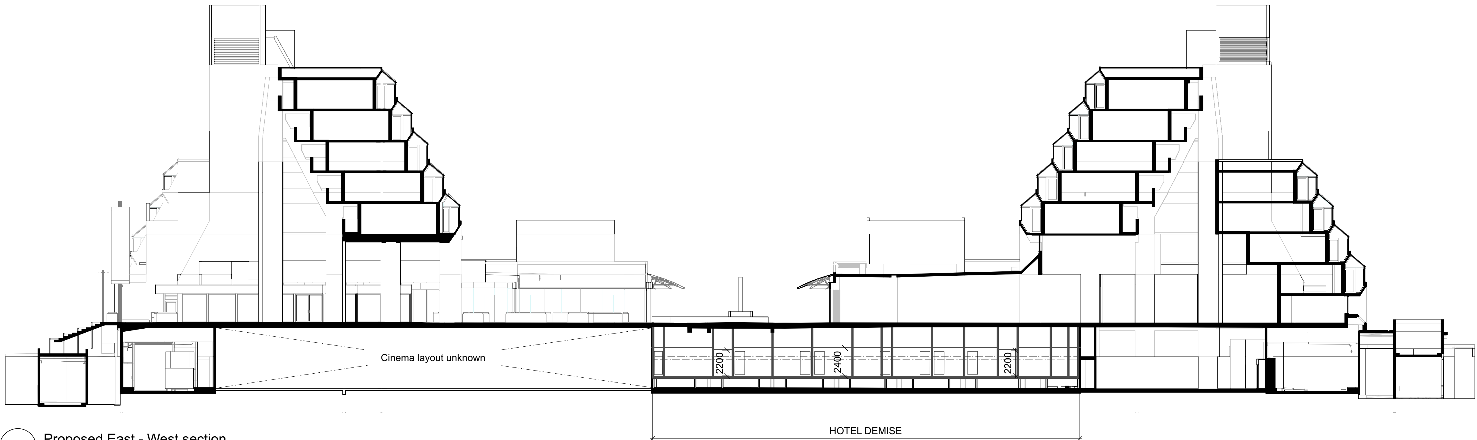
2 Proposed East - West section Scale: 1:200
