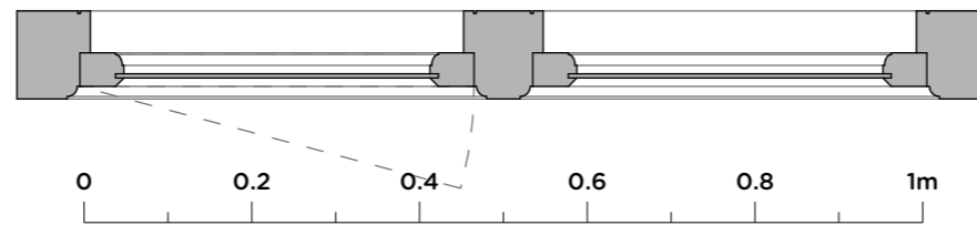
02 EXISTING PLAN E(PA)W02 1:10@A3
