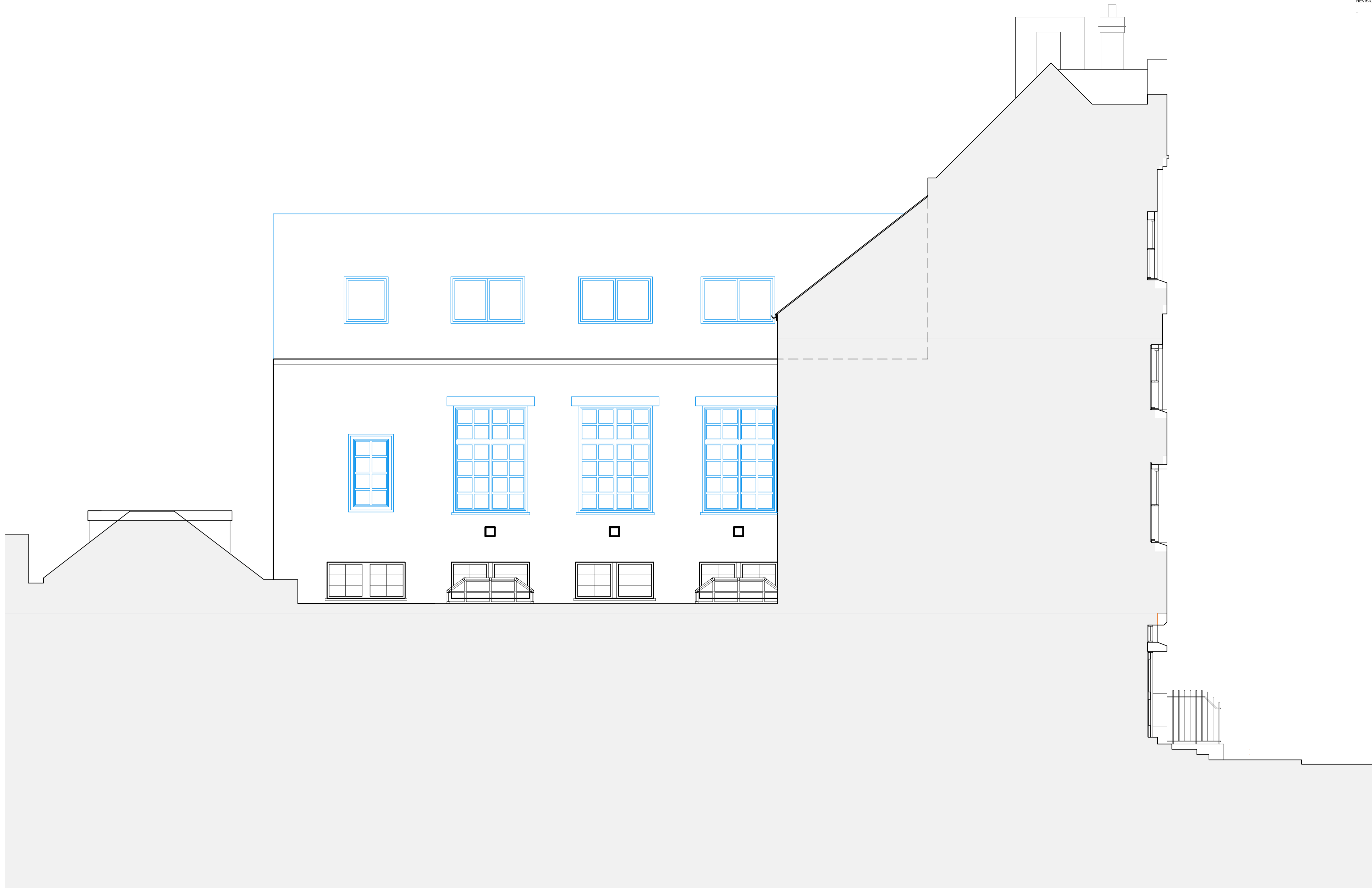
South Elevation
