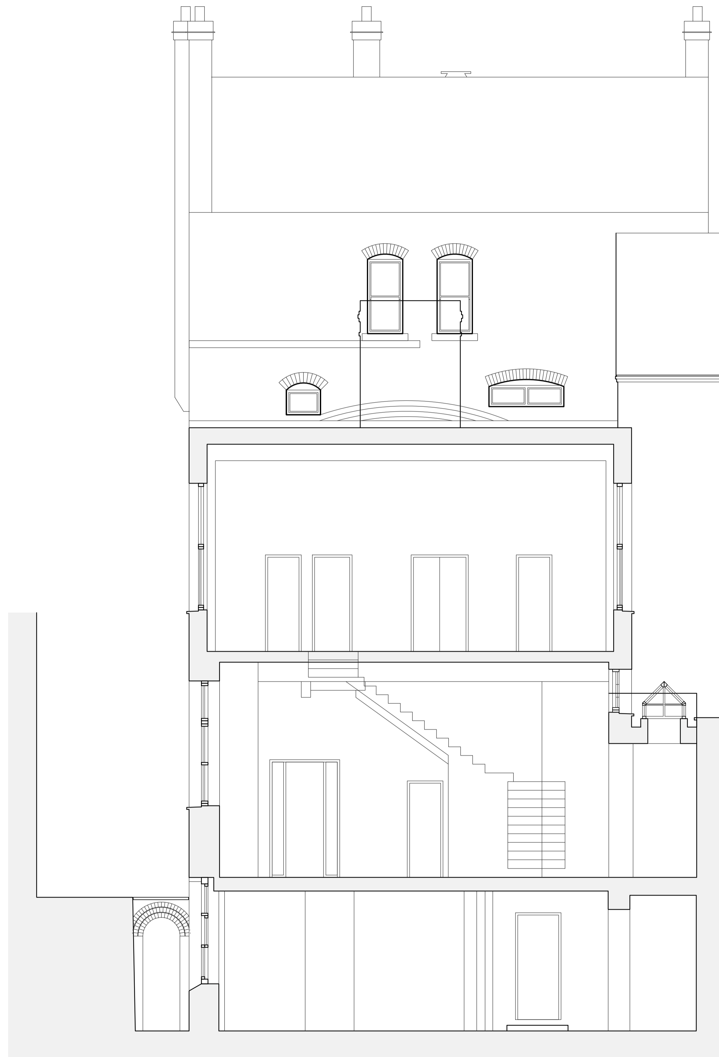
Cross Section (looking east)
