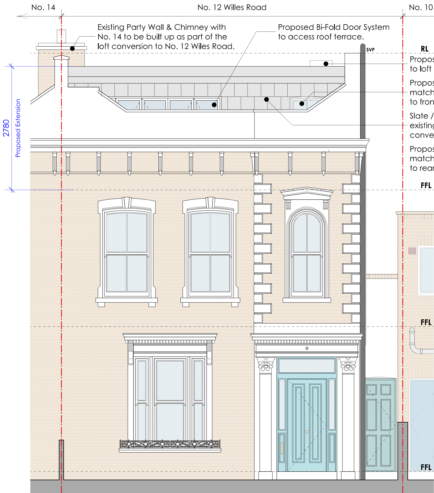
1 Proposed Front Elevation scale: 1:50 @ A3
