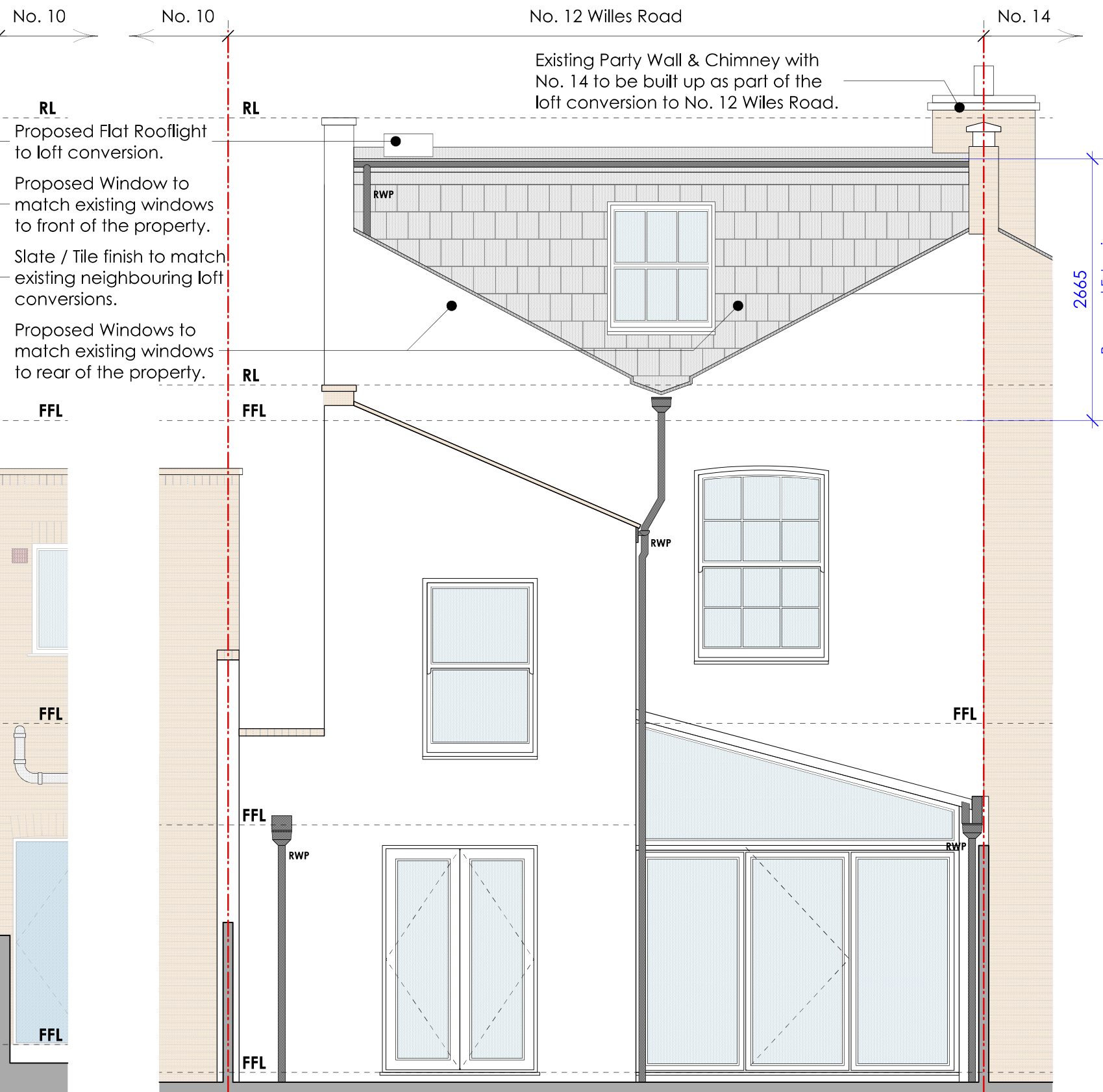
2 Proposed Rear Elevation scale: 1:50 @ A3
