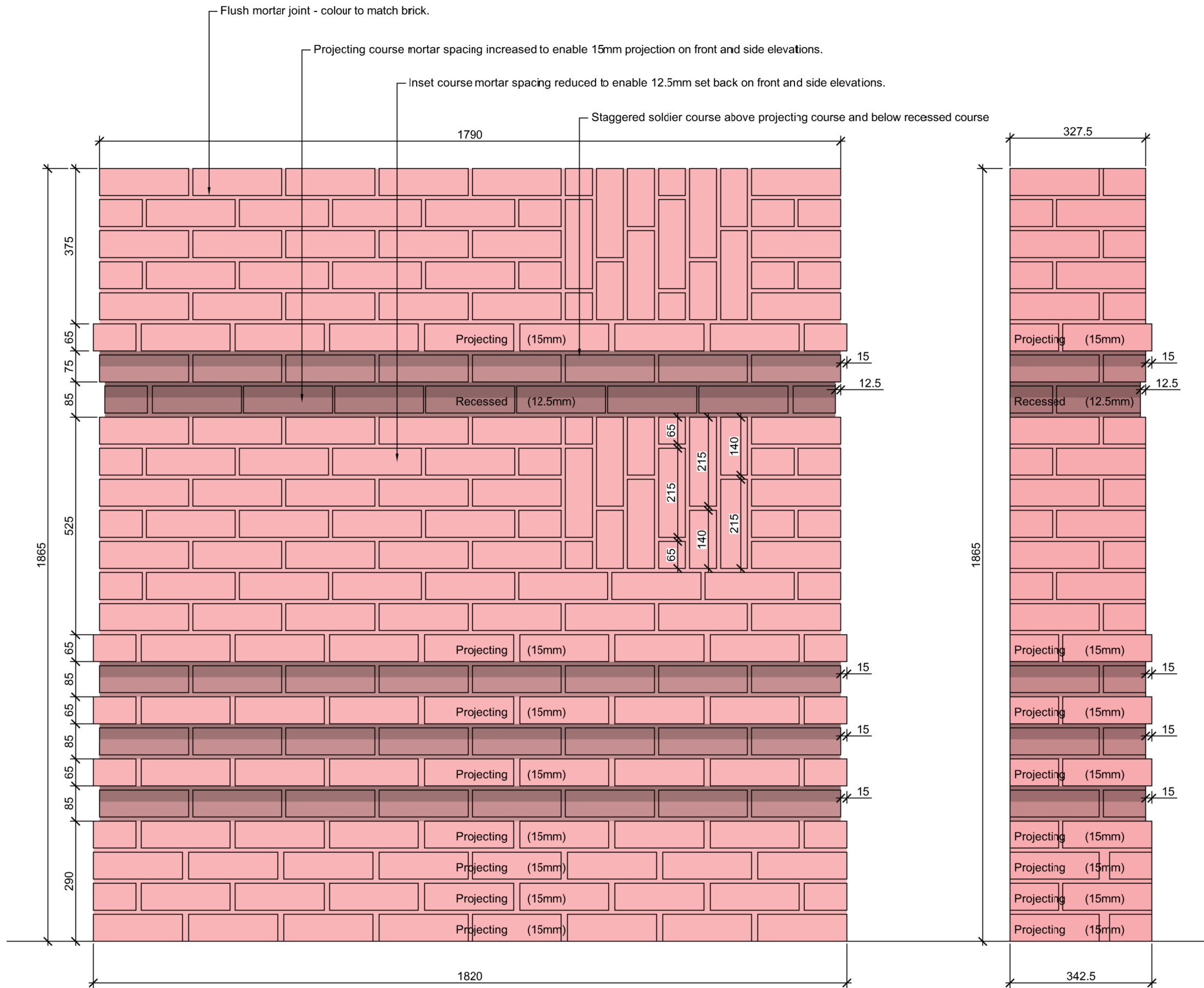
Front Elevation
