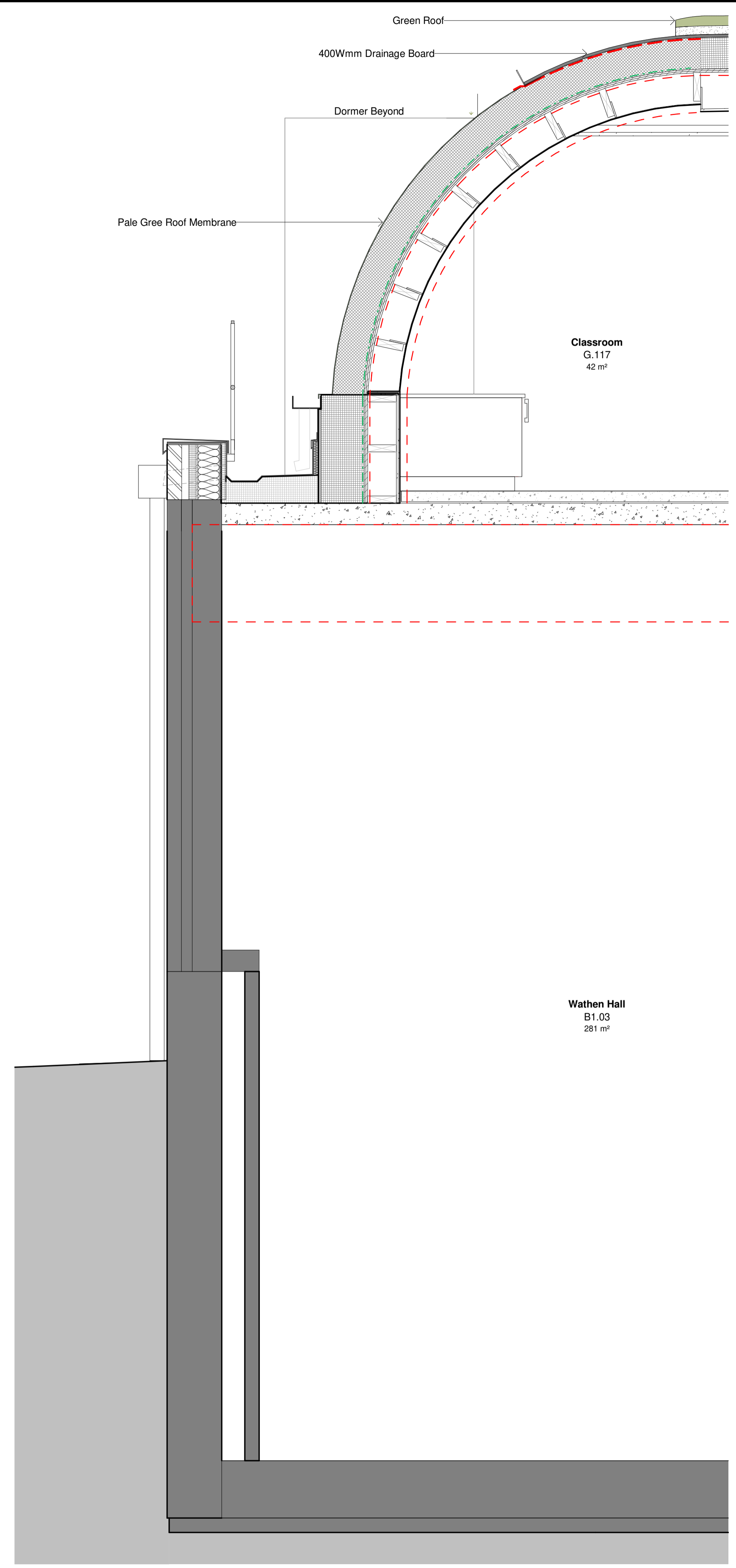
ENLARGED SECTION A - 01 1 : 20
