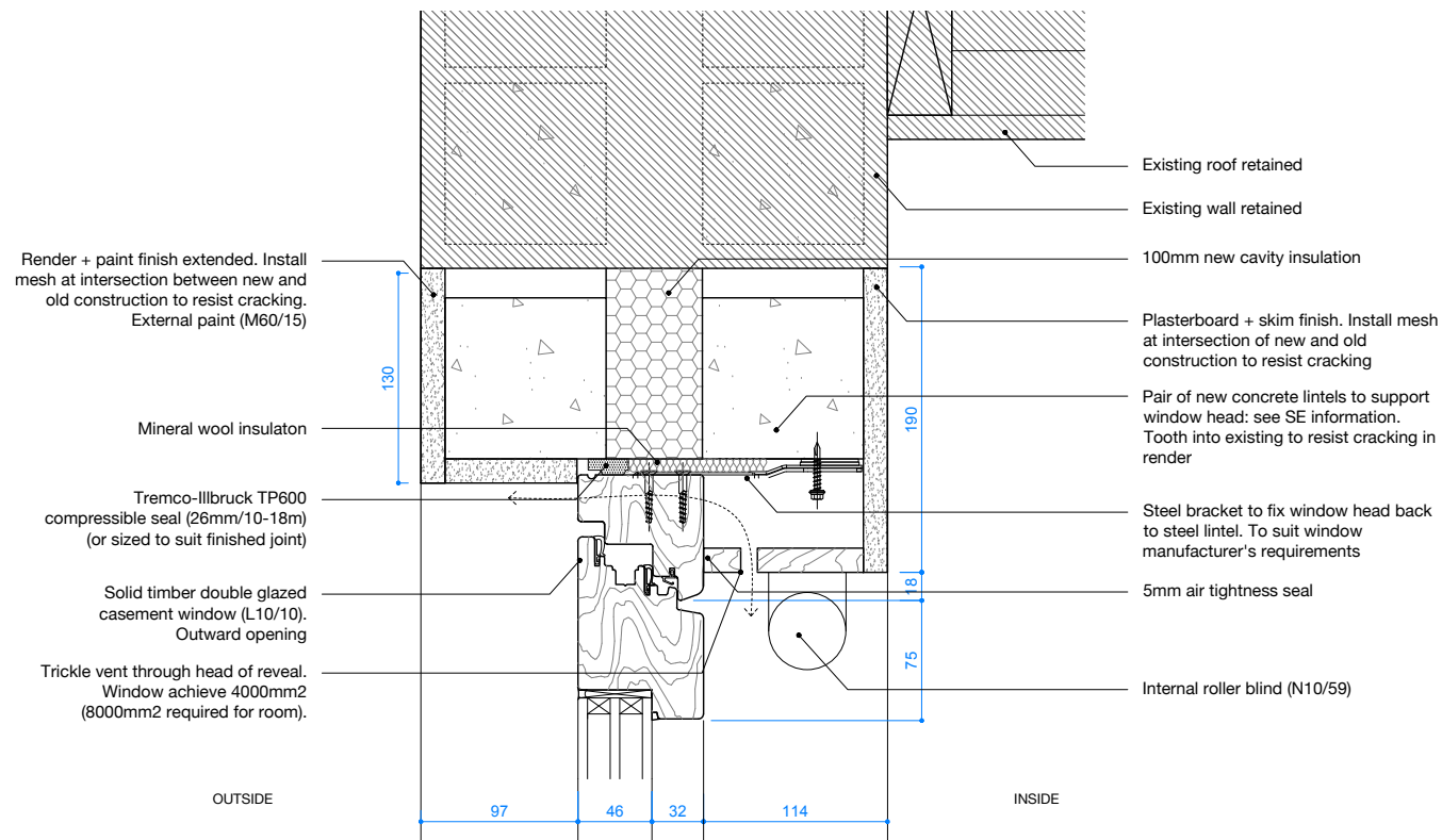
D01_Window Head
