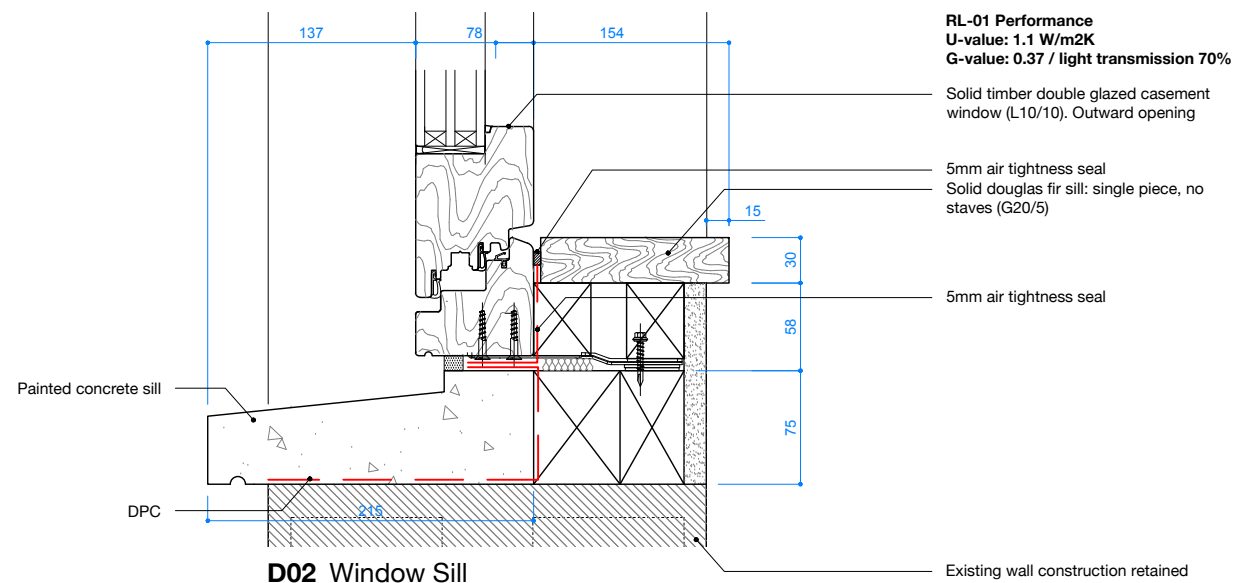
D02_Window Sill
