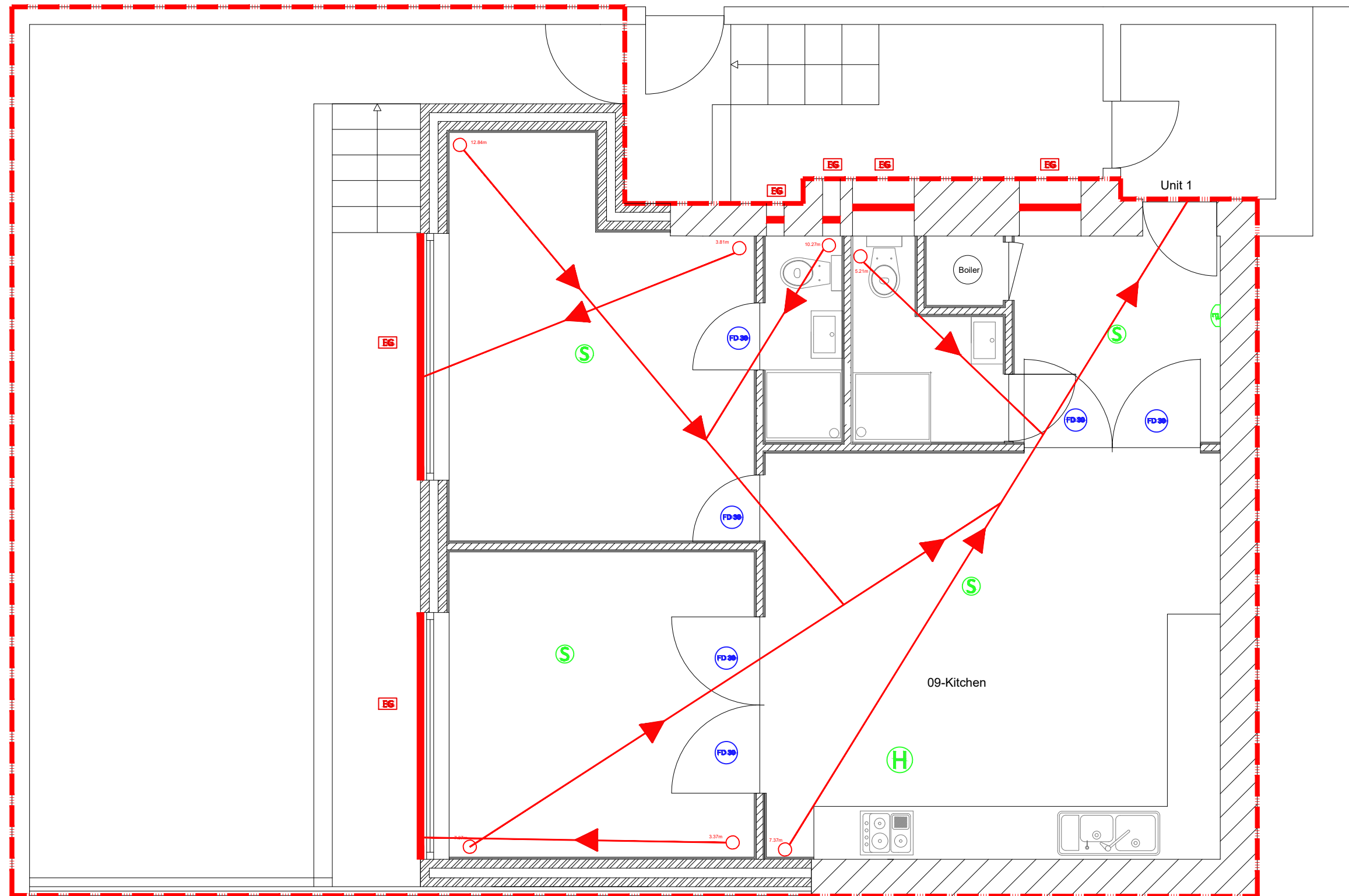
Proposed Lower Ground floor Fire Strategy
