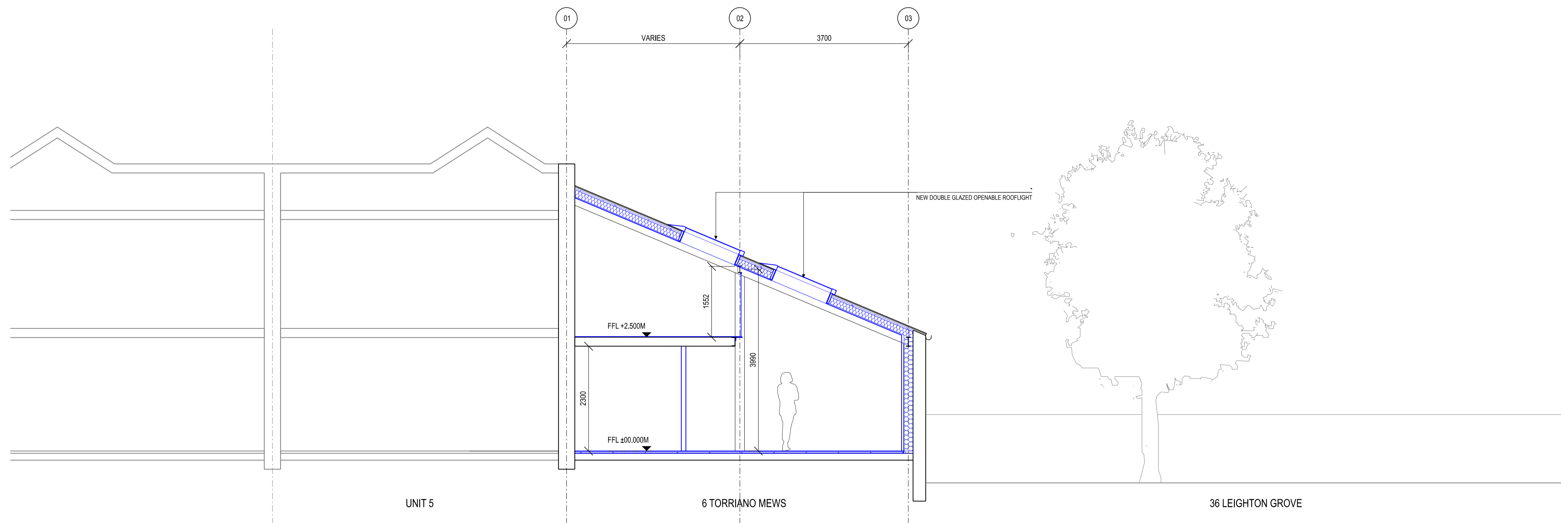
02 PROPOSED CROSS SECTION 1:50@A1
