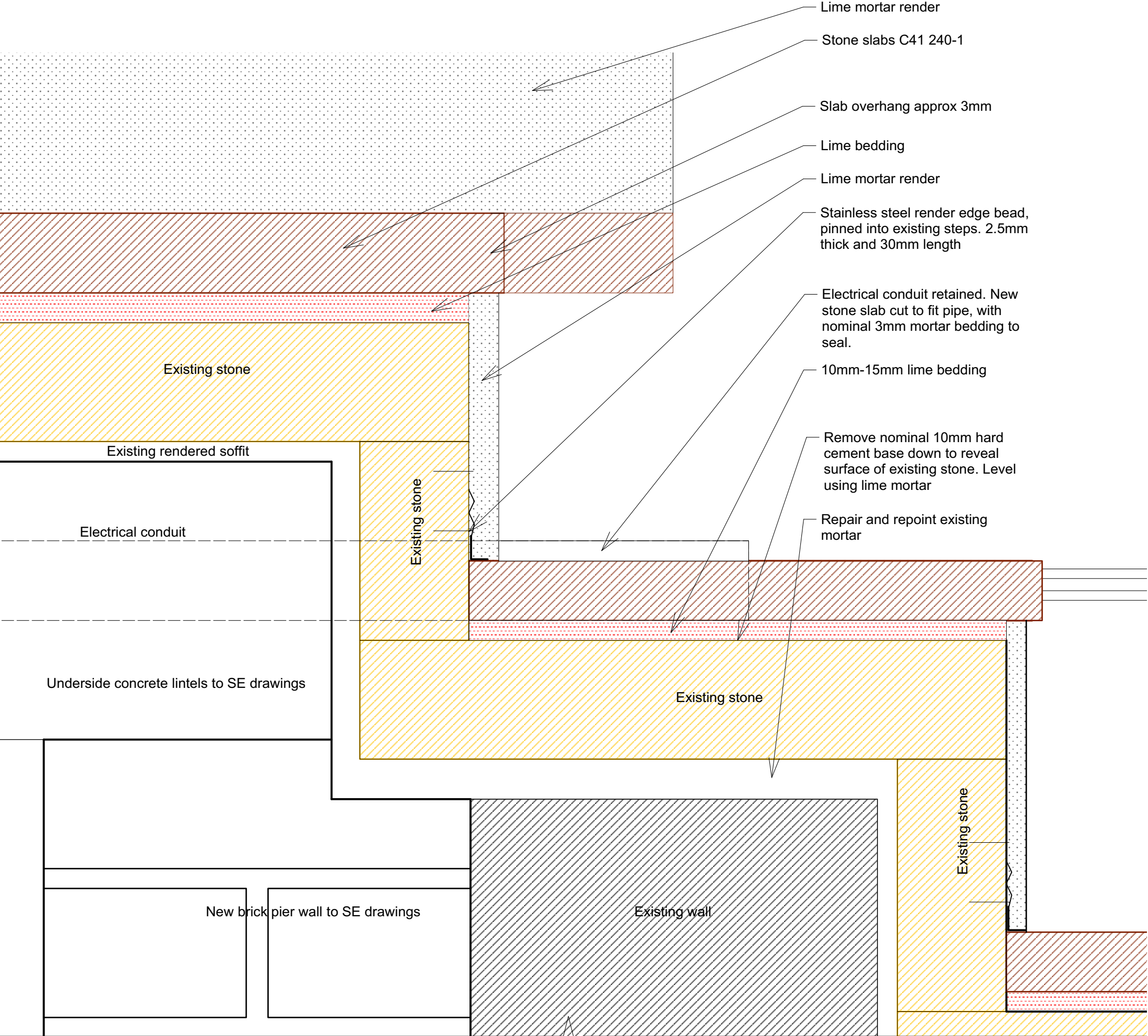
Section Detail B 1:2
