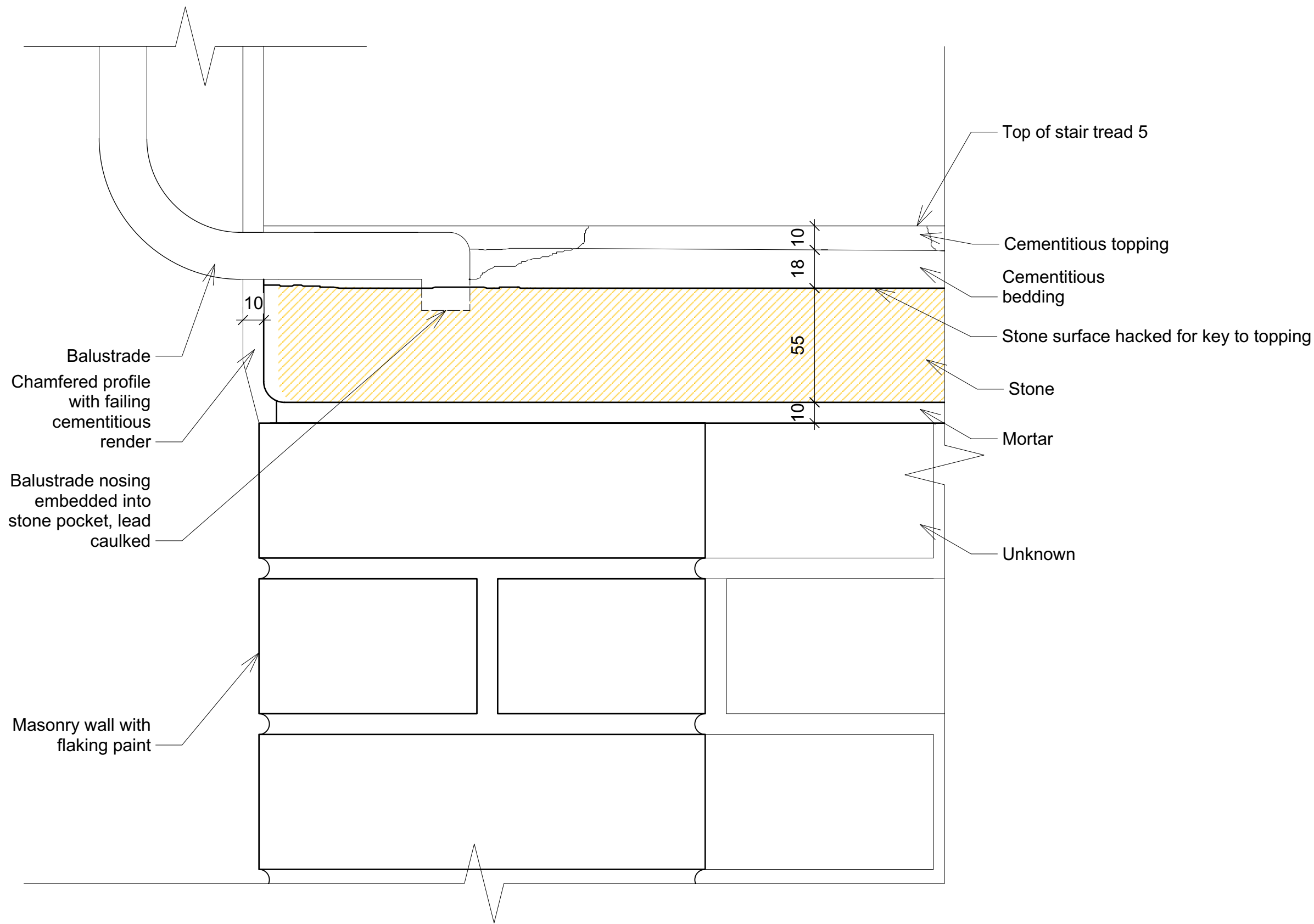
Staircase 03 - Section Detail E
