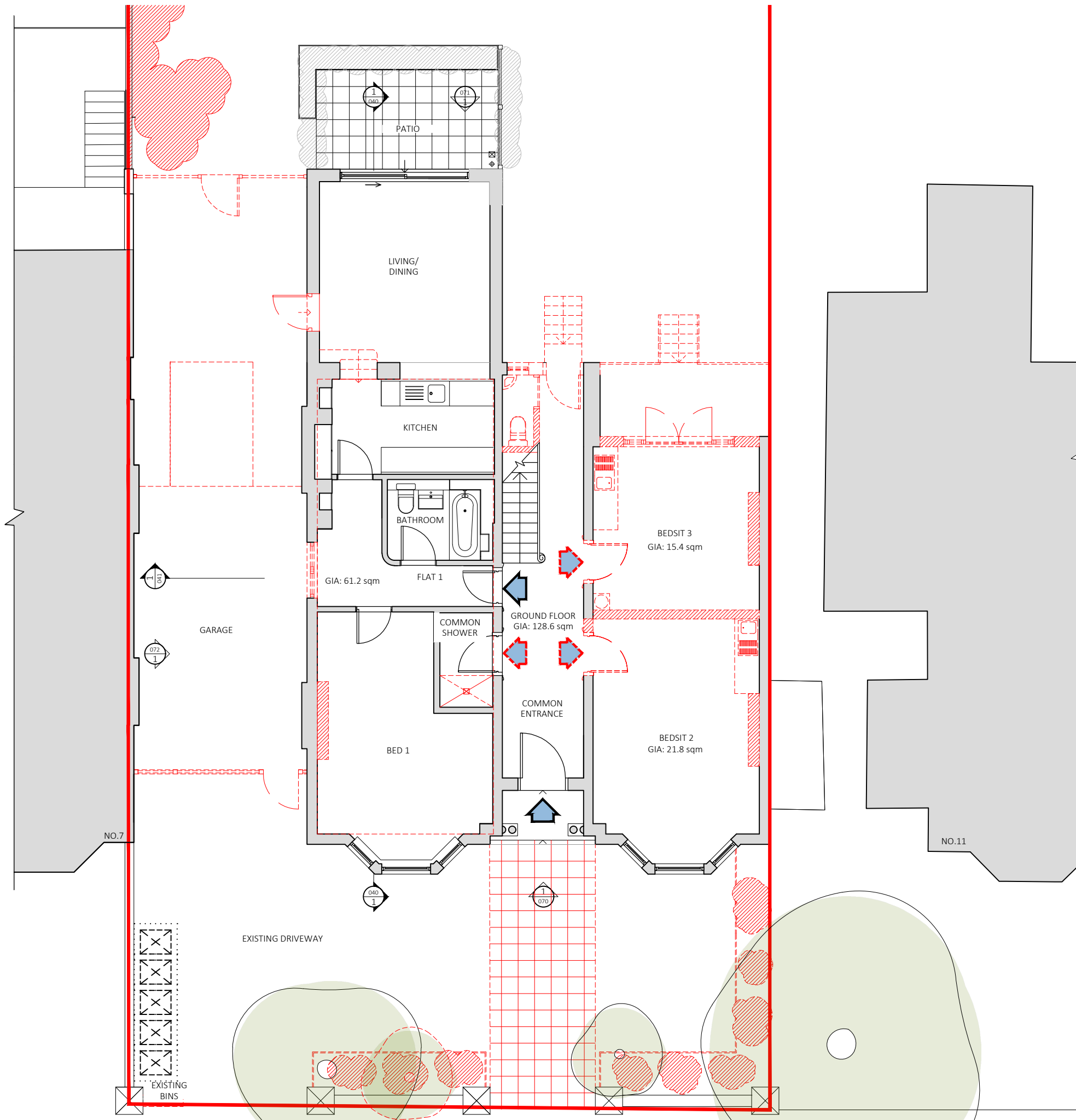
1 EXISTING GROUND FLOOR DEMO PLAN 1:100 @ A3
