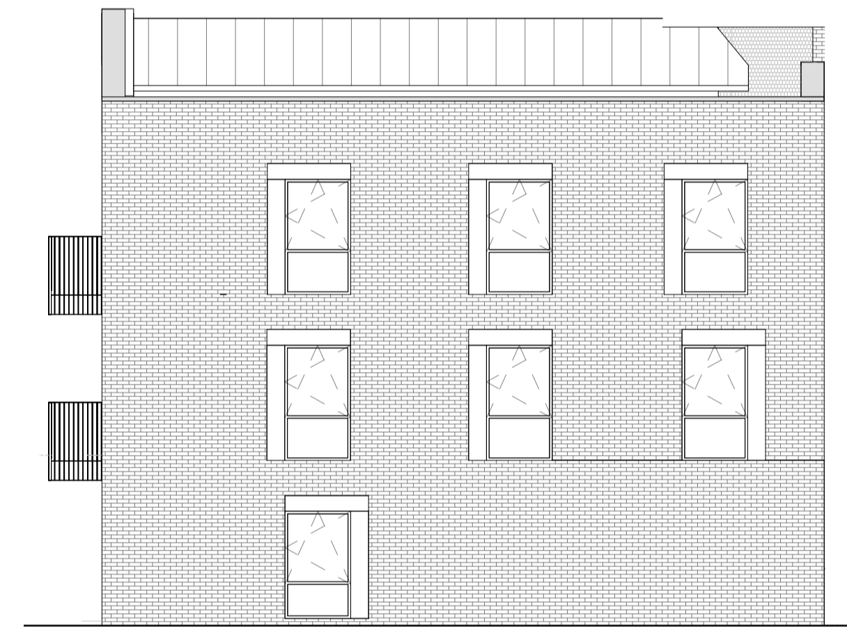
7 | Plot 6 - Elevation 07 1:100
