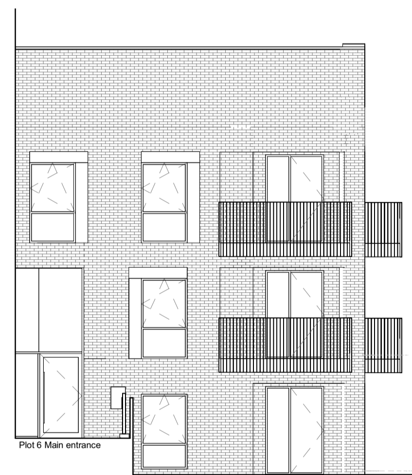
5 | Plot 6 - Elevation 05 1:100
