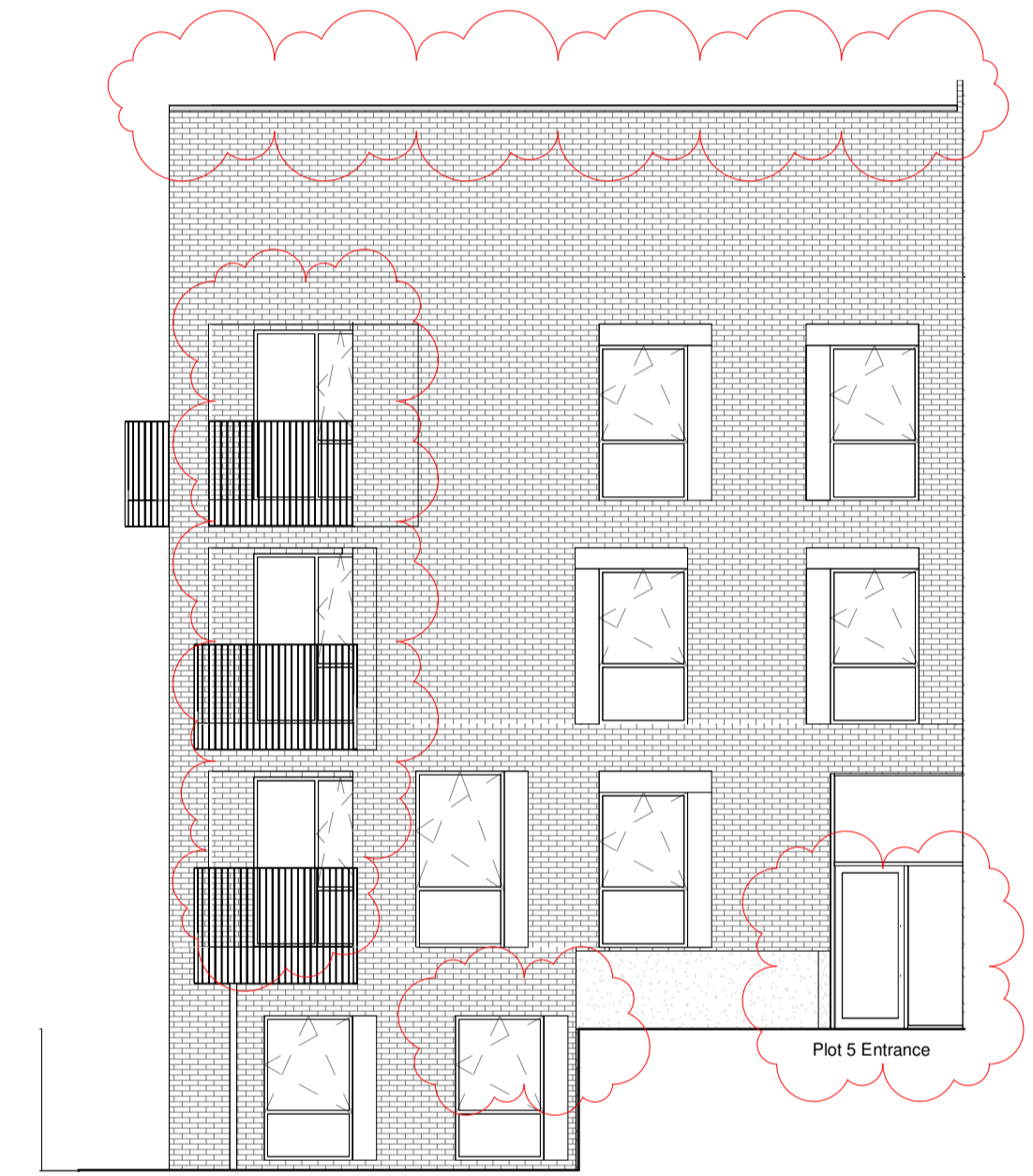
4 | Plot 5 - Elevation 04 1:100
