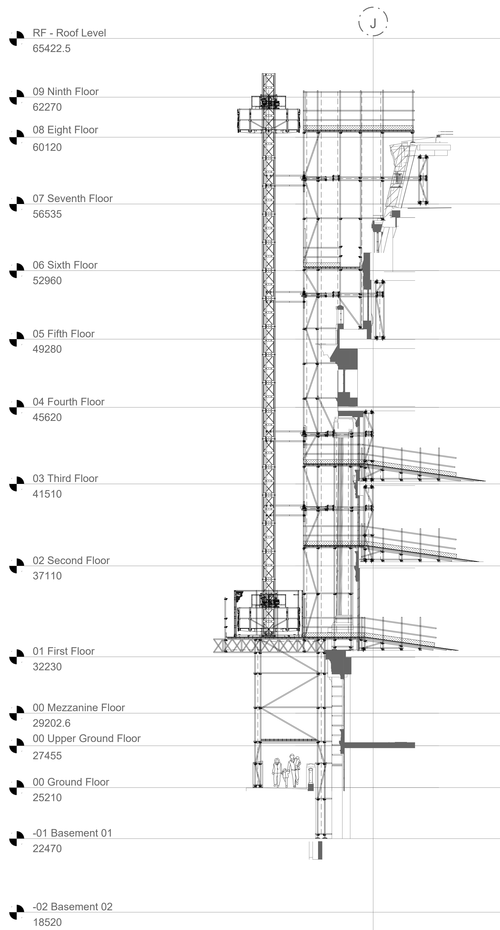
A Section - Proposed Hoist - Section A 1 : 100
