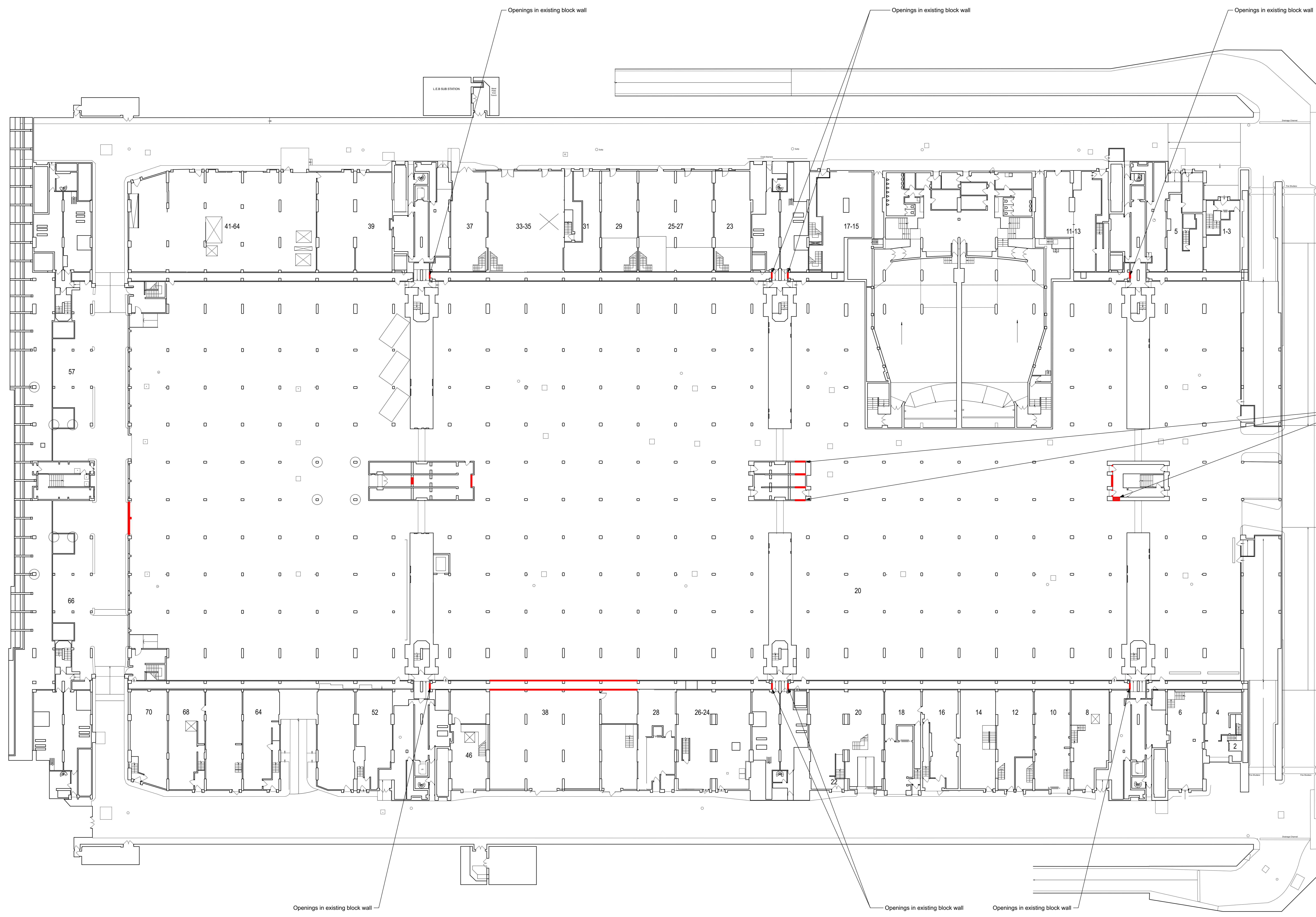
1 Fabric Removal Plan - Lower basement Scale: 1:200
