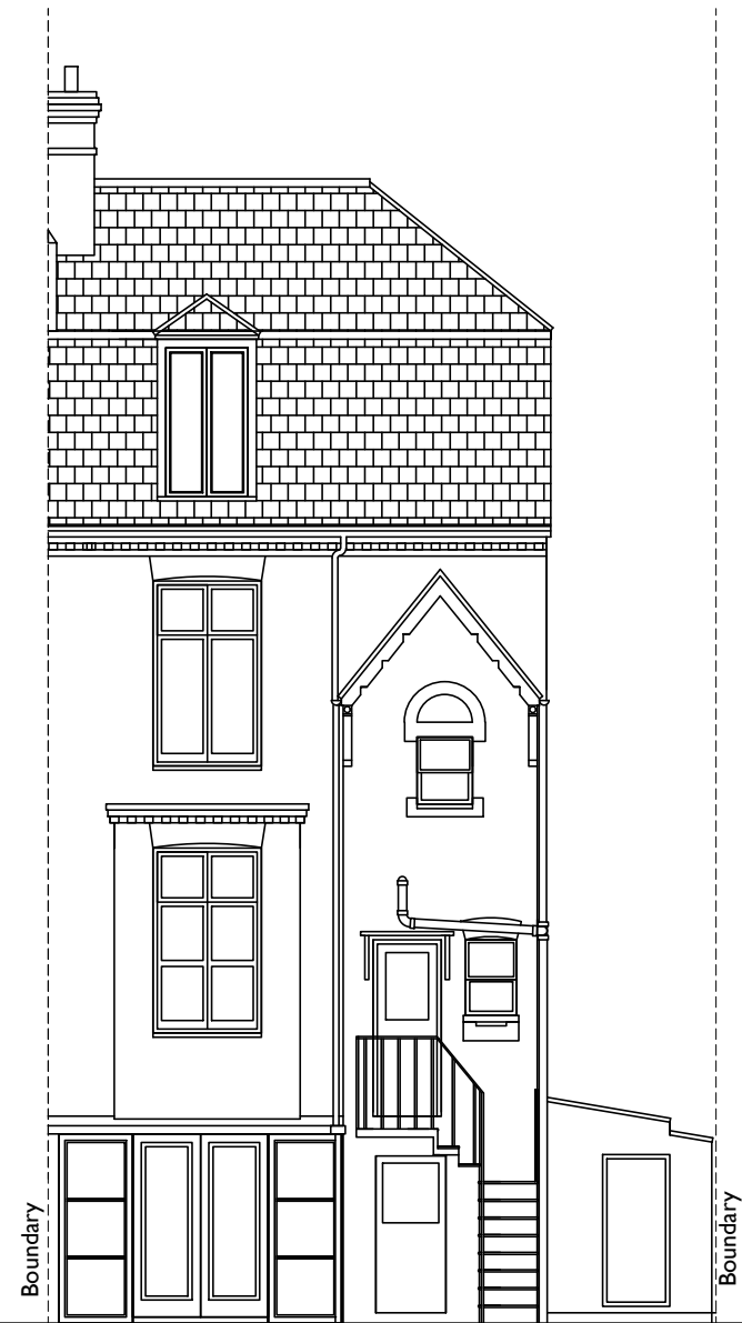
REAR ELEVATION
