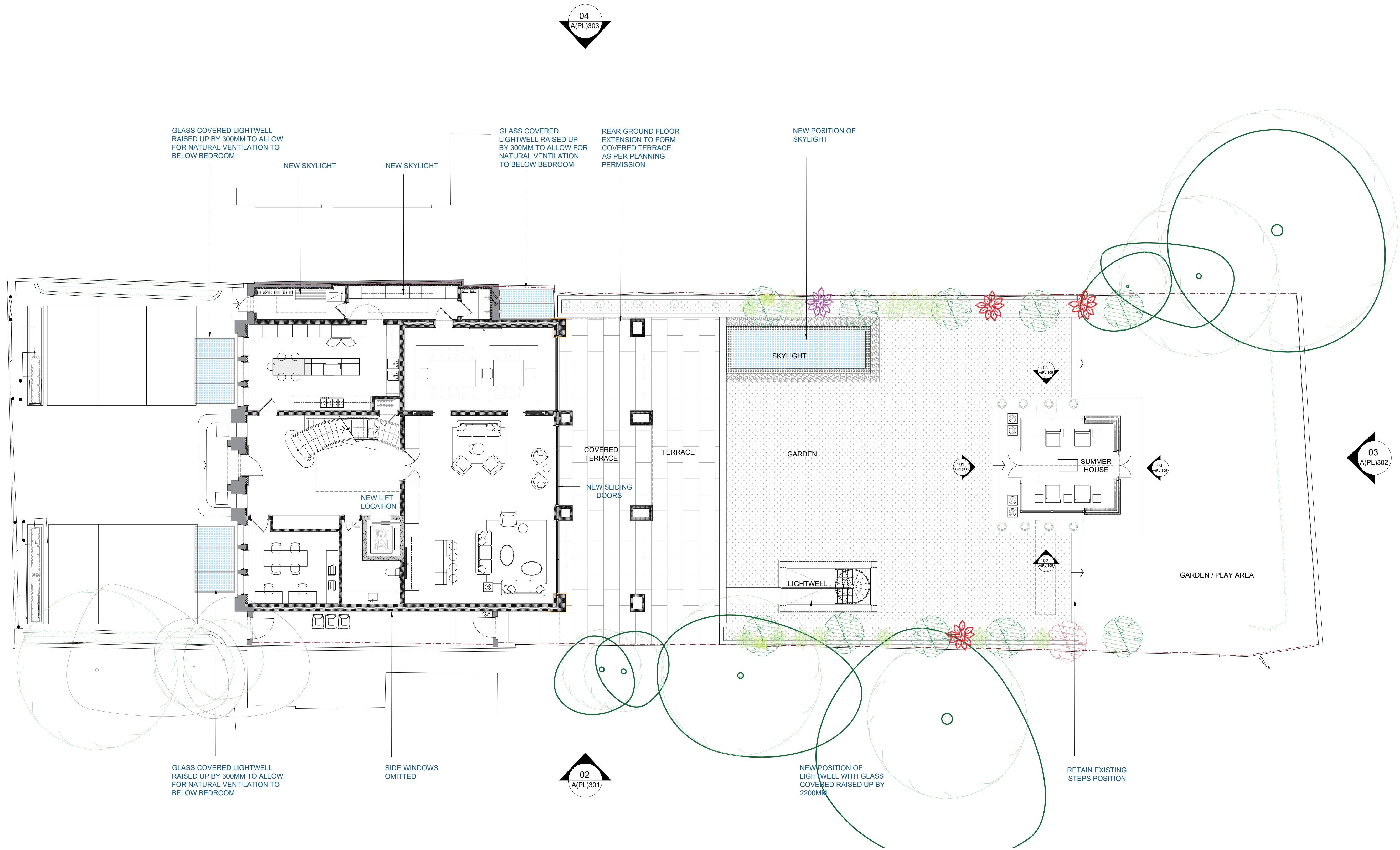
Si SITE PLAN - GROUND FLOOR SCALE 1:100 @ A1
