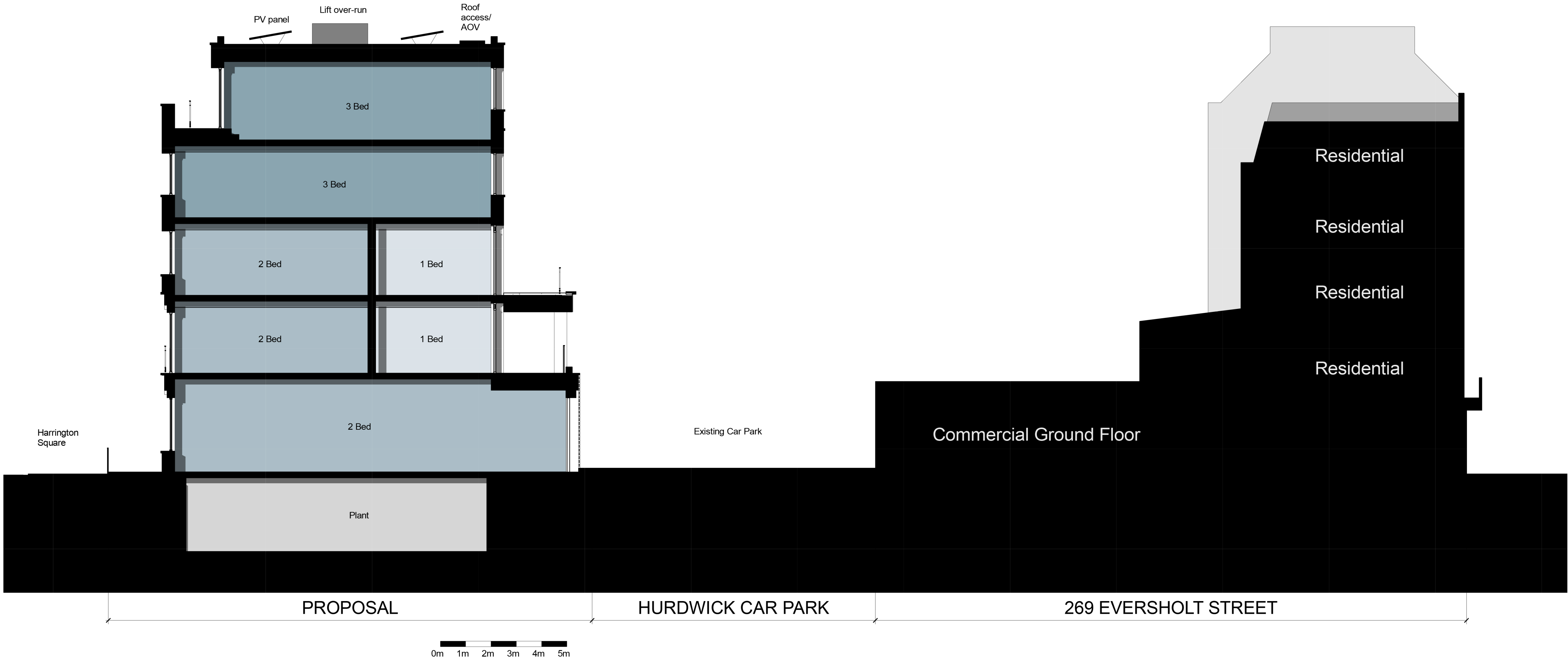
2 Proposed Building Section 1 : 100
