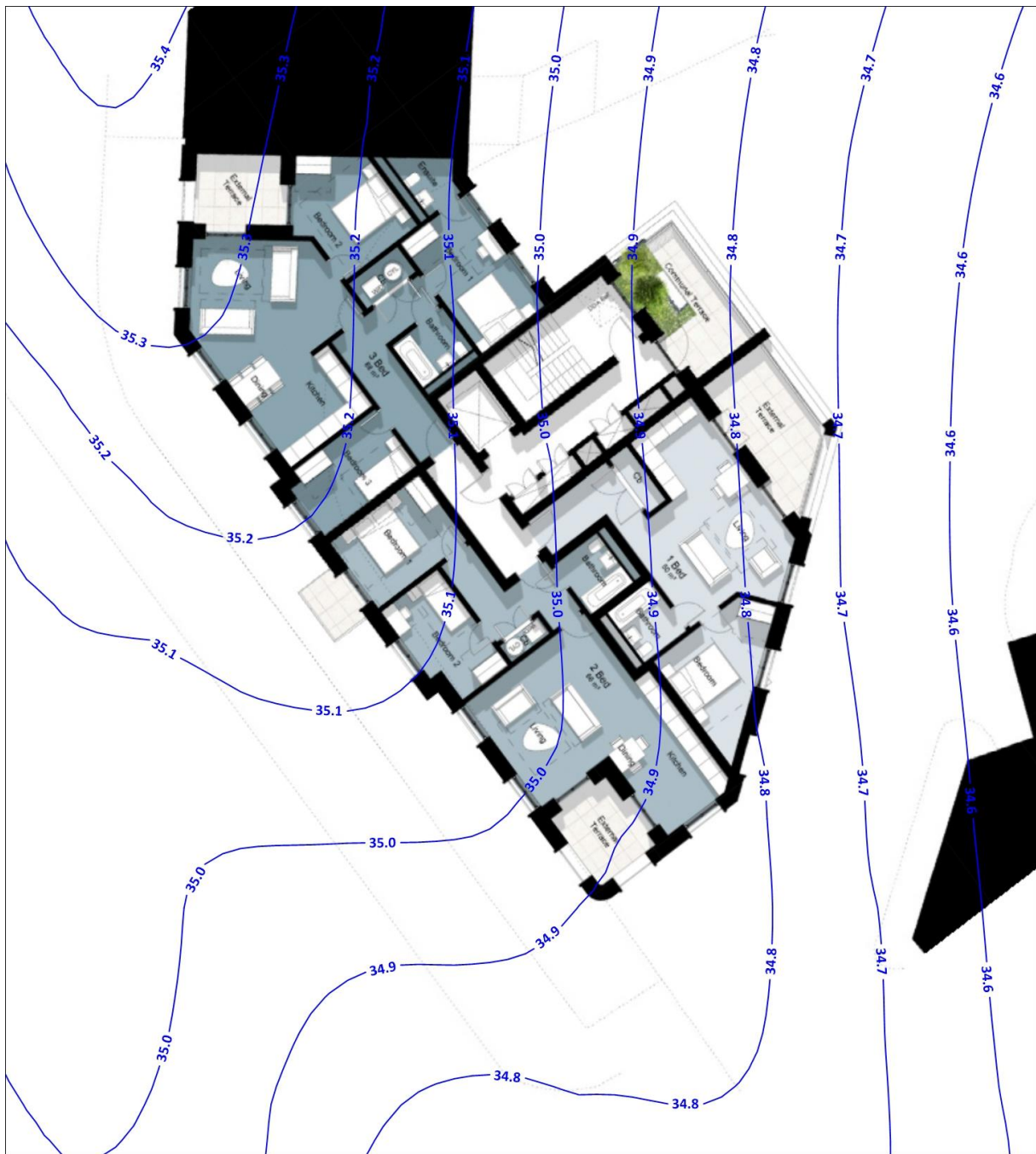
Figure 6: Predicted 2025 First-Floor Level Annual Mean NO 2 Concentrations (µg/m 3 )
