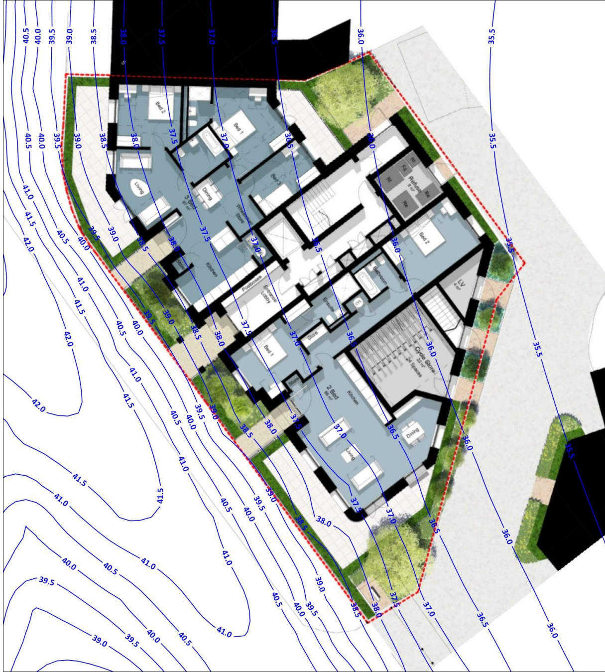
Figure 5: Predicted 2025 Ground-Floor Level Annual Mean NO 2 Concentrations (µg/m 3 )
