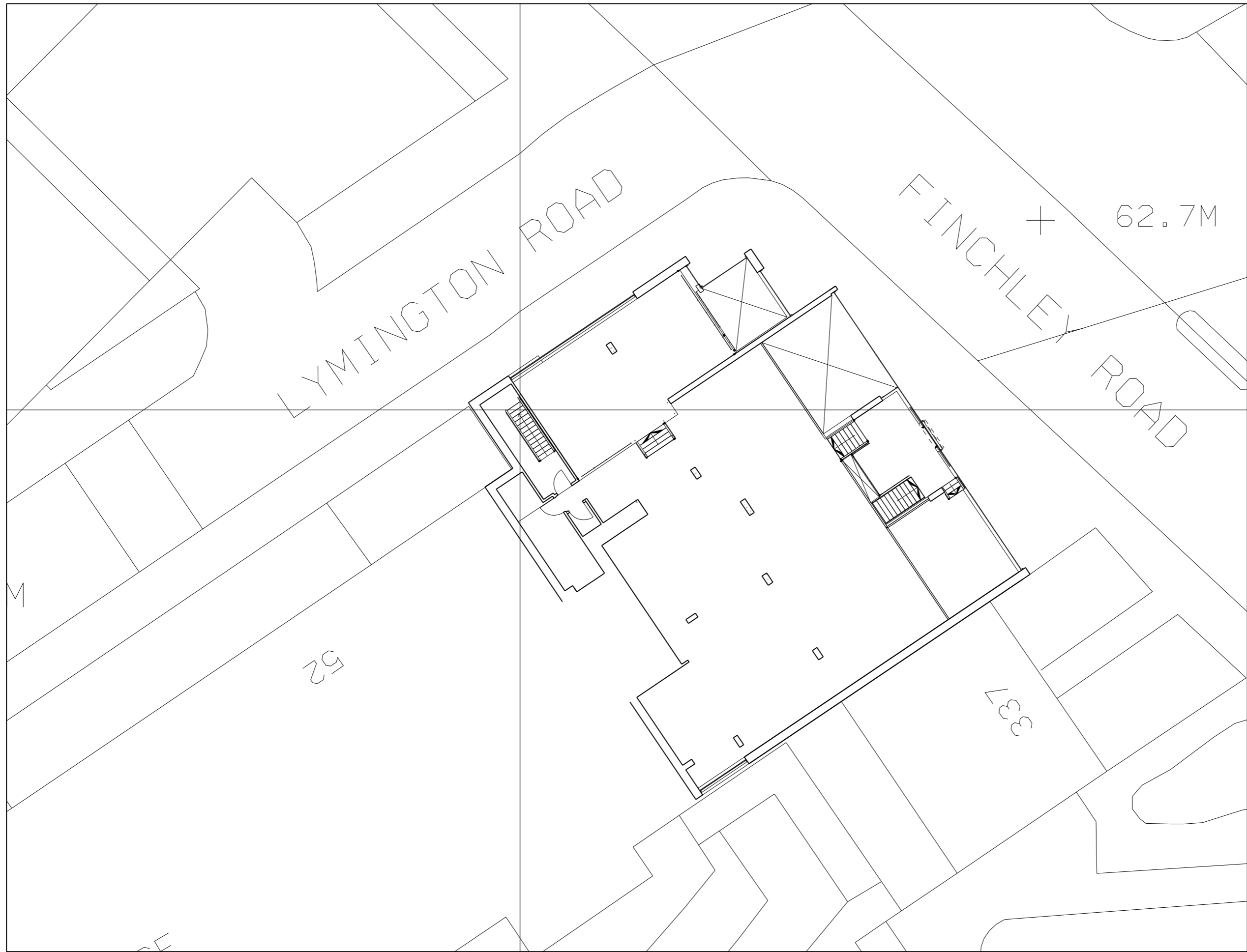
01 EXISTING SITE PLAN: UPPER GROUND FLOOR SCALE 1:200
