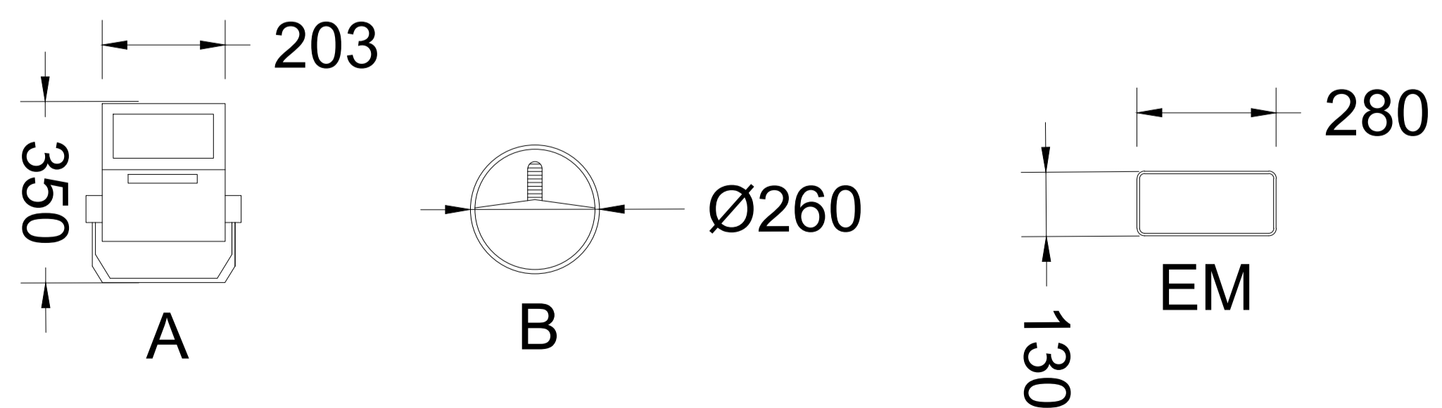
LUMINAIRE DIMENSIONS NTS @ A1
