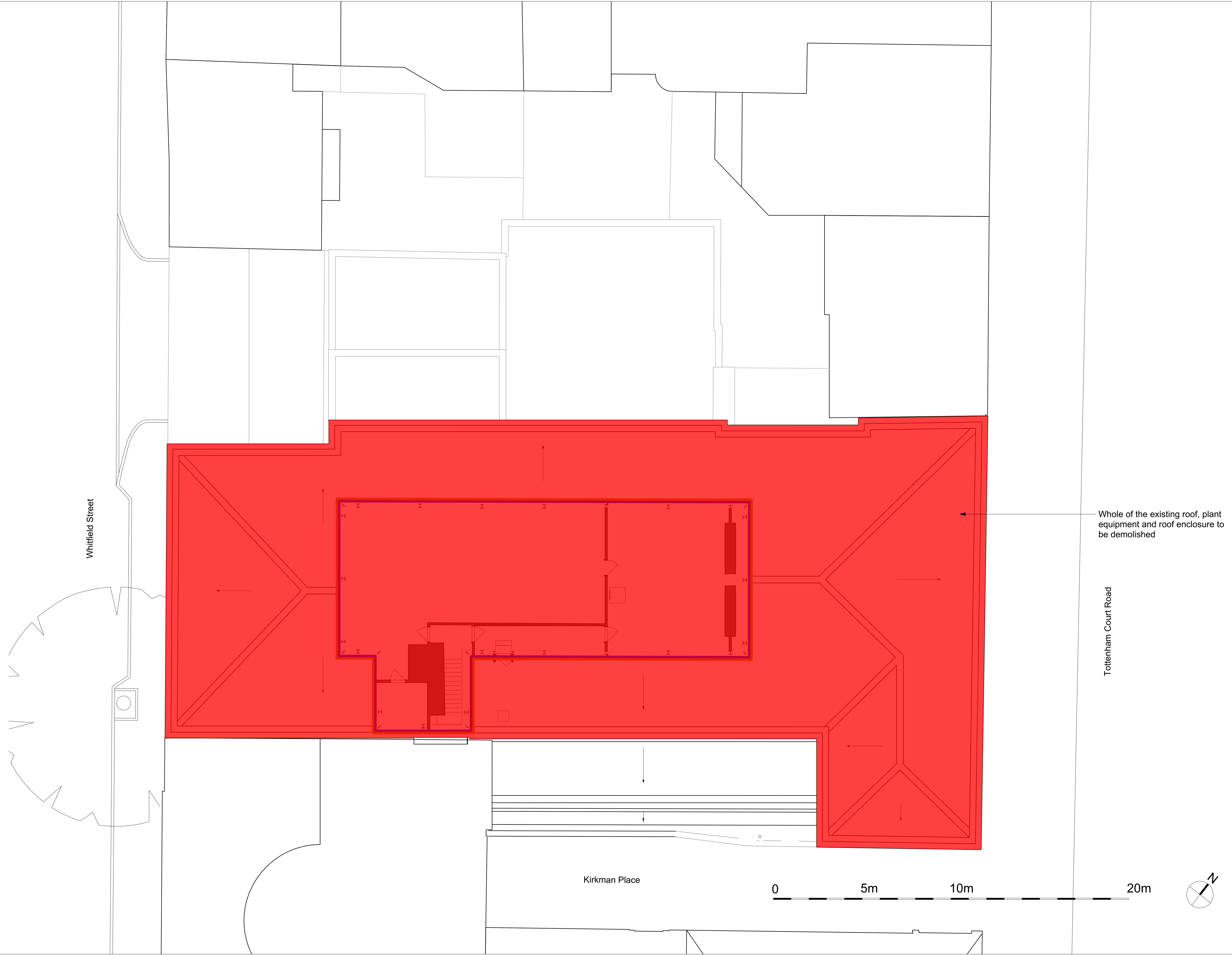
1 Roof Demolition Plan Scale: 1:100
