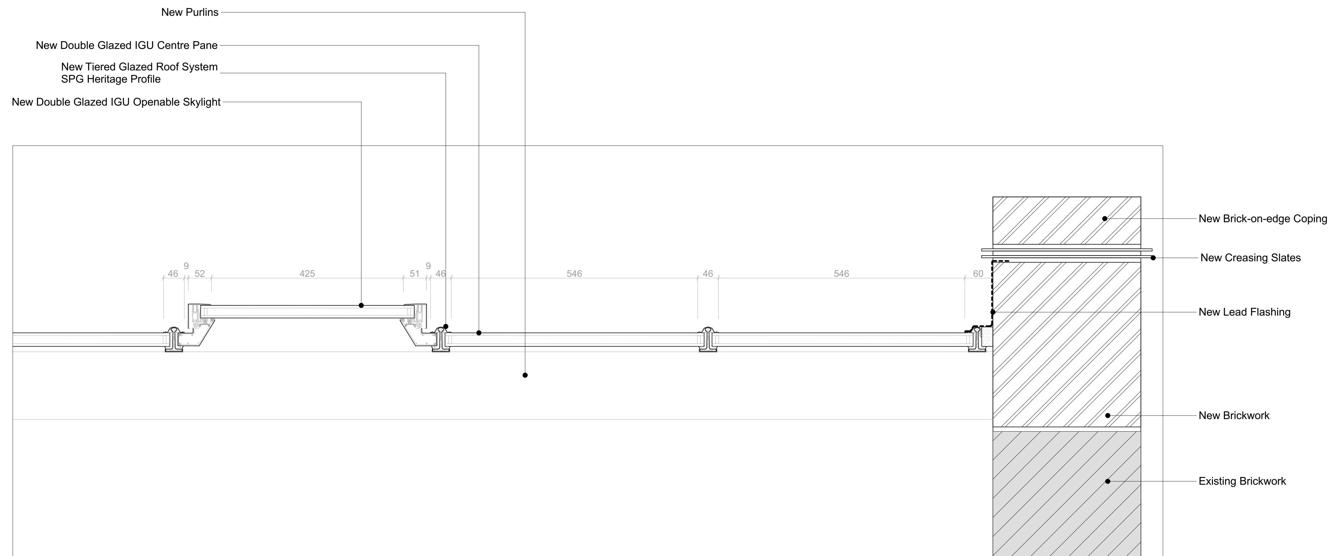
01 Proposed Glazed Opening 7013 1:5 @ A1
