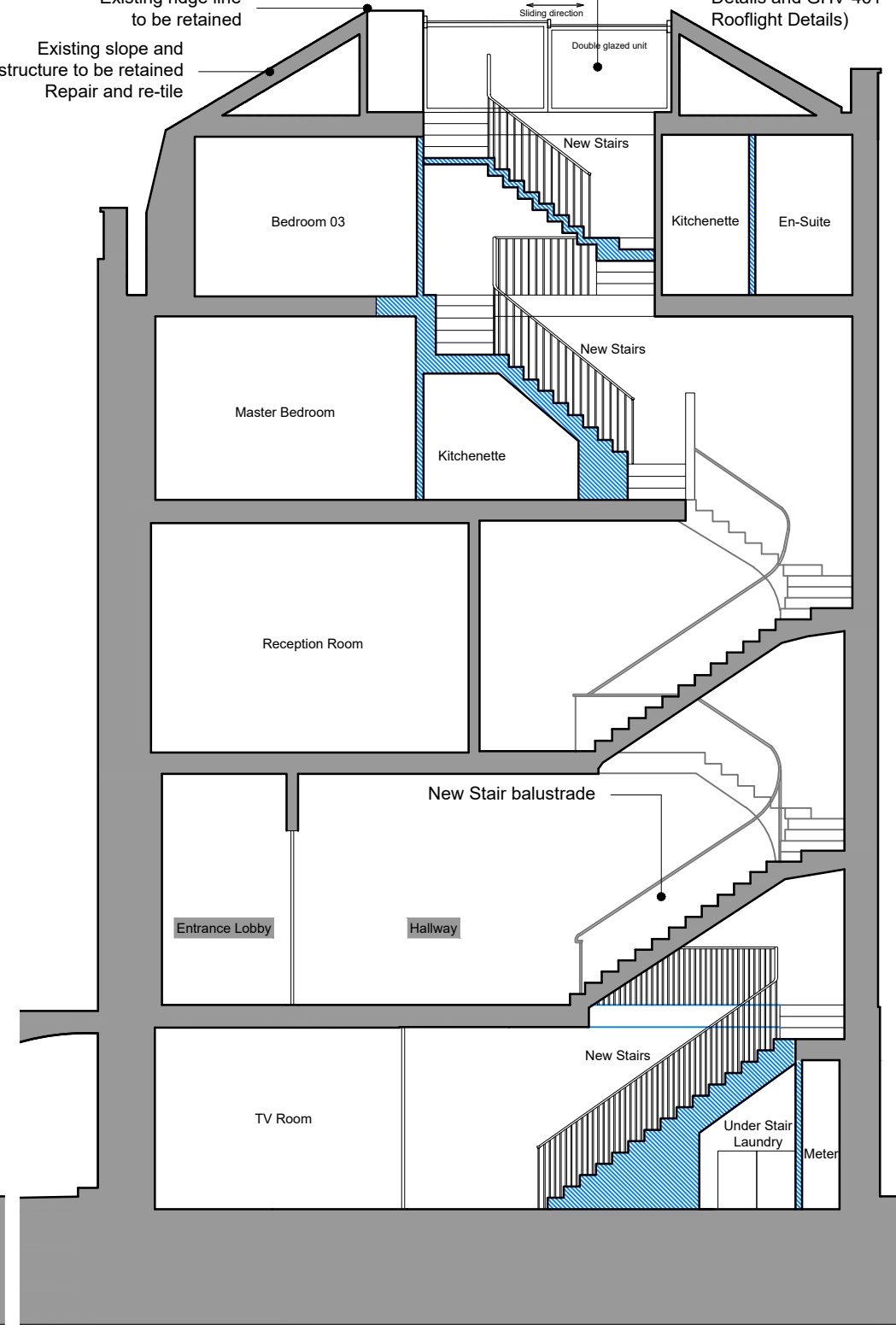
3 Proposed Section B-B GHV 1:100 @ A3
