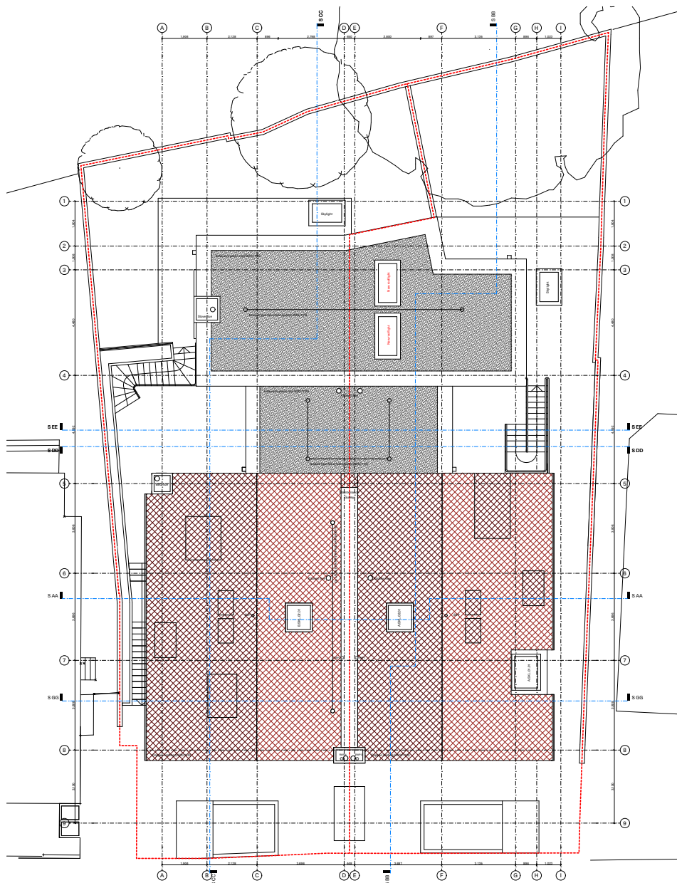
Roof Plan - Consented
