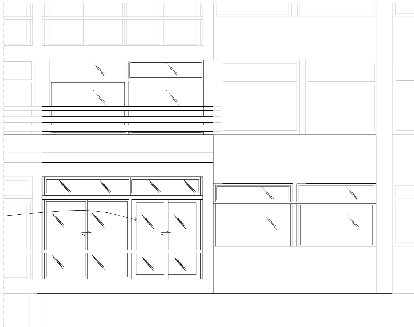
Flat 9 - Proposed External Elevation (see dwg cph ew 009 to locate on main elevation)
