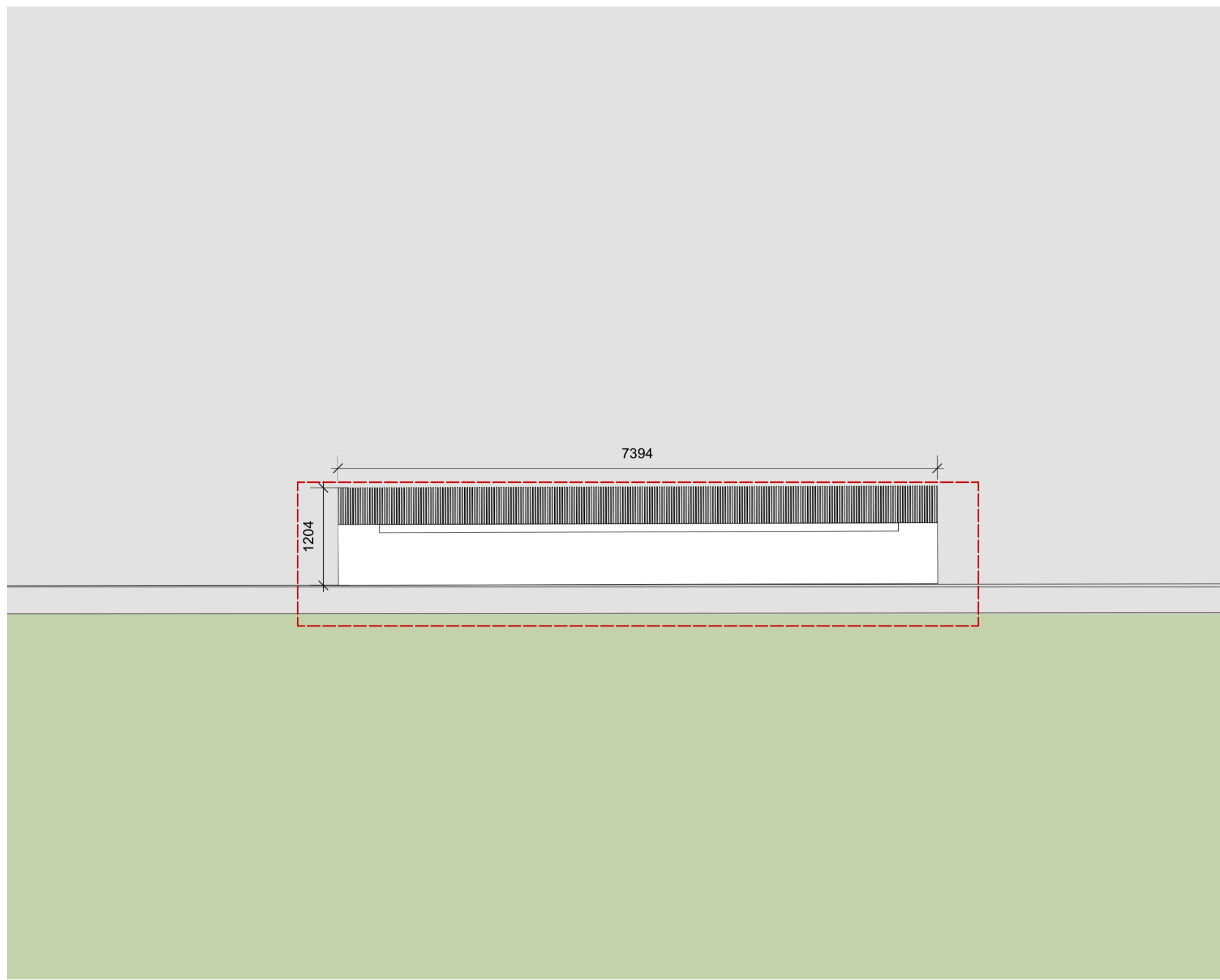
1 Social Screen - Proposed Scale: 1:50
