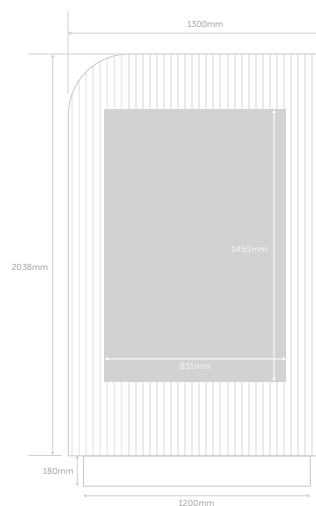
REAR ELEVATION
