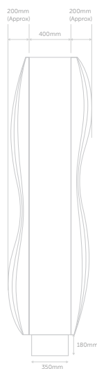
SIDE ELEVATION
