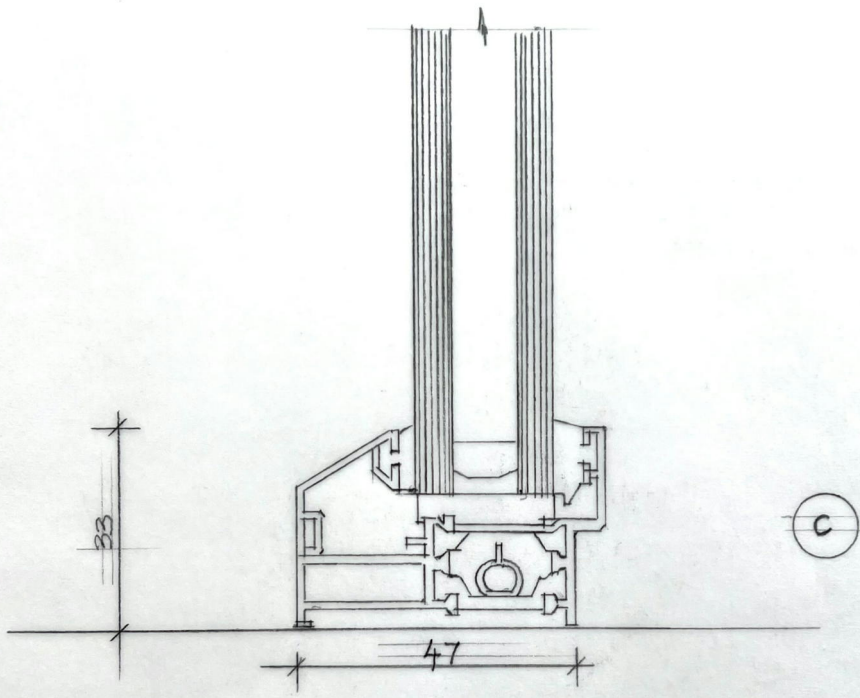
SECTION 'E' HERITAGE FIXED CILL LIGHT SECTION
