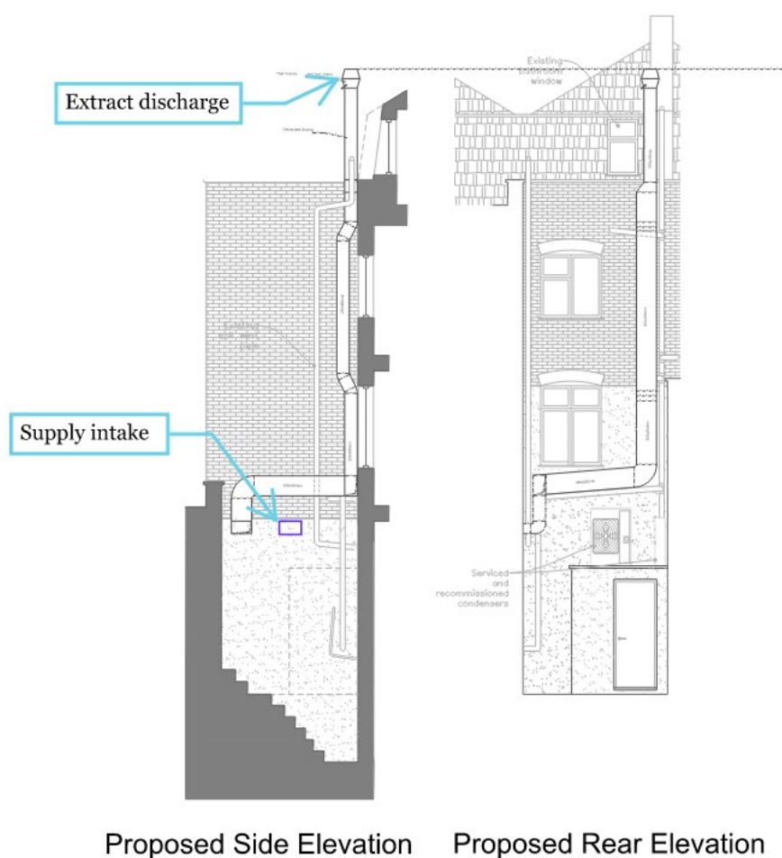
Figure 3 Elevations
