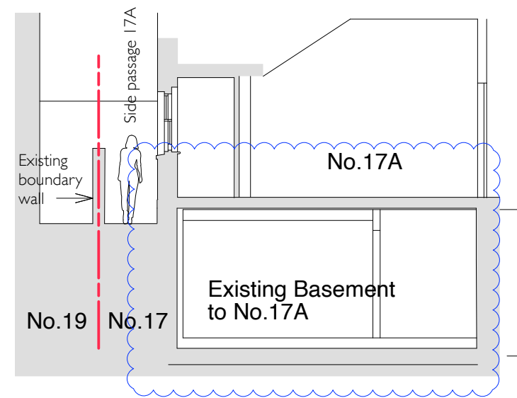
2 Section BB As Proposed Scale 1:100
