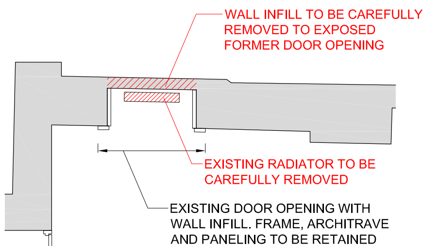
1 GROUND FLOOR - AS EXISTING & DEMOLITIONS 55-59 GORDON SQUARE 1:20 @ A1
