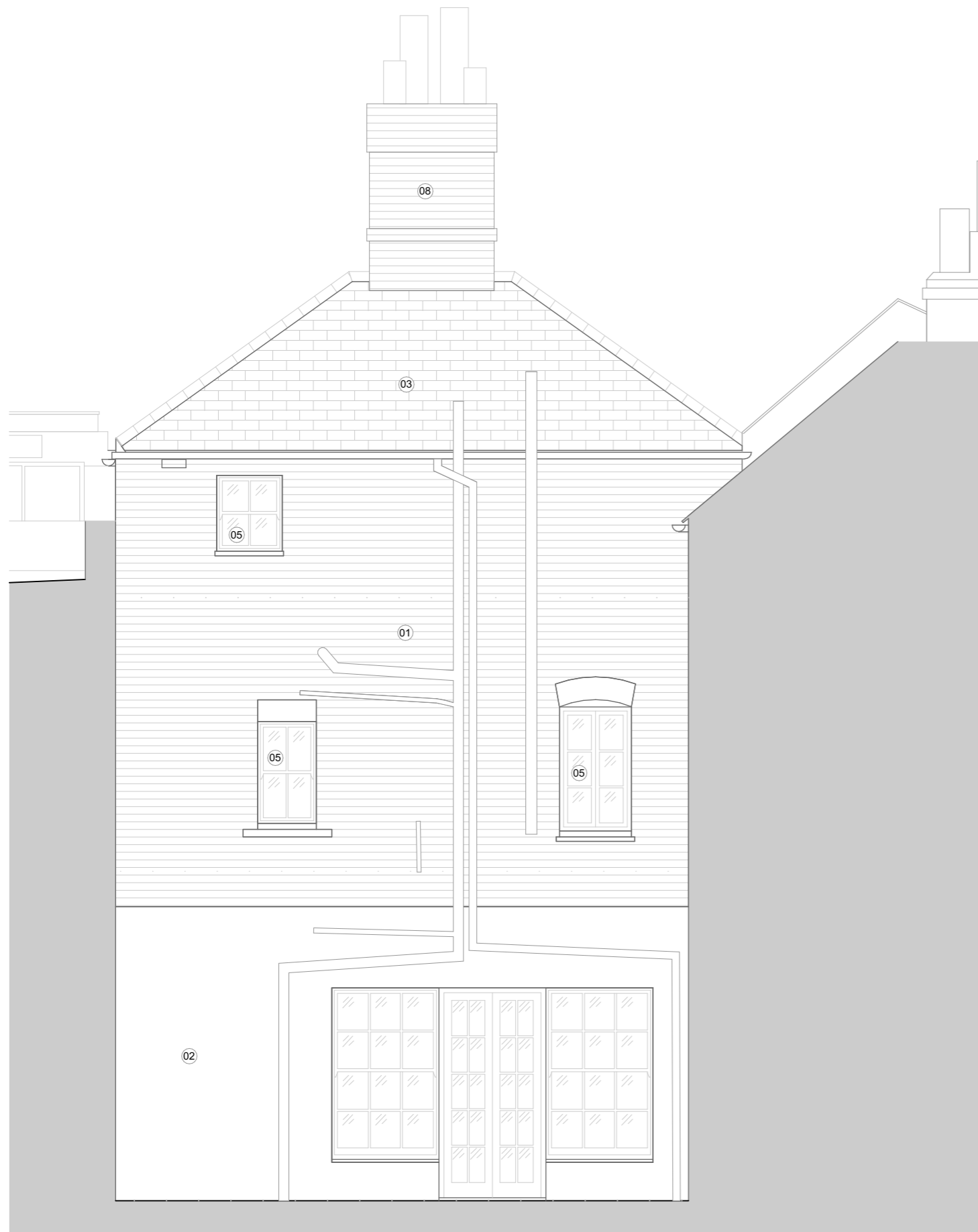
NORTHWEST ELEVATION AS PROPOSED
