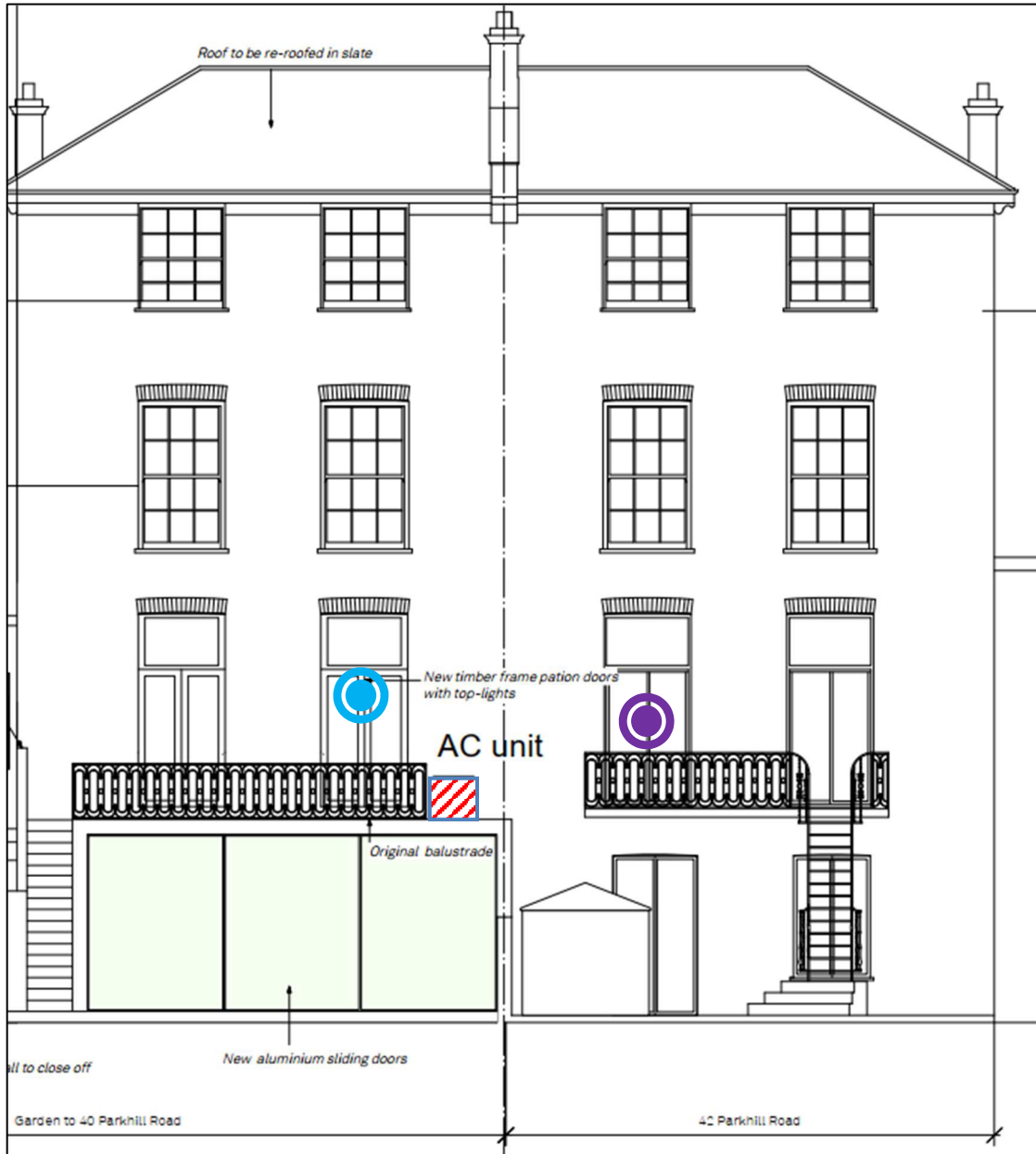
Figure 2.5 Site measurement position, identified receiver and proposed plant unit installation (Image Source: Paul Archer Design)
