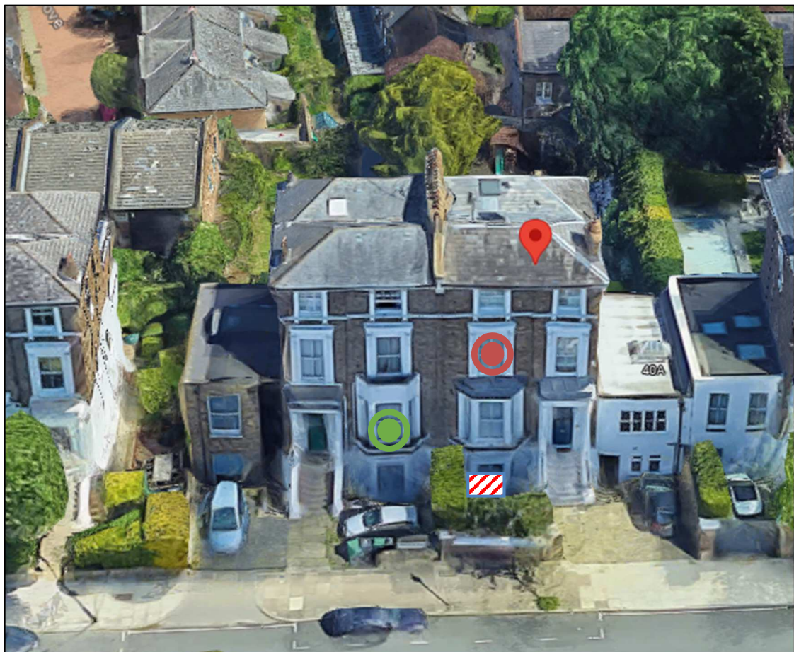
Figure 2.2 Site measurement position, identified receiver and proposed plant unit installation (Image Source: Google Maps)
