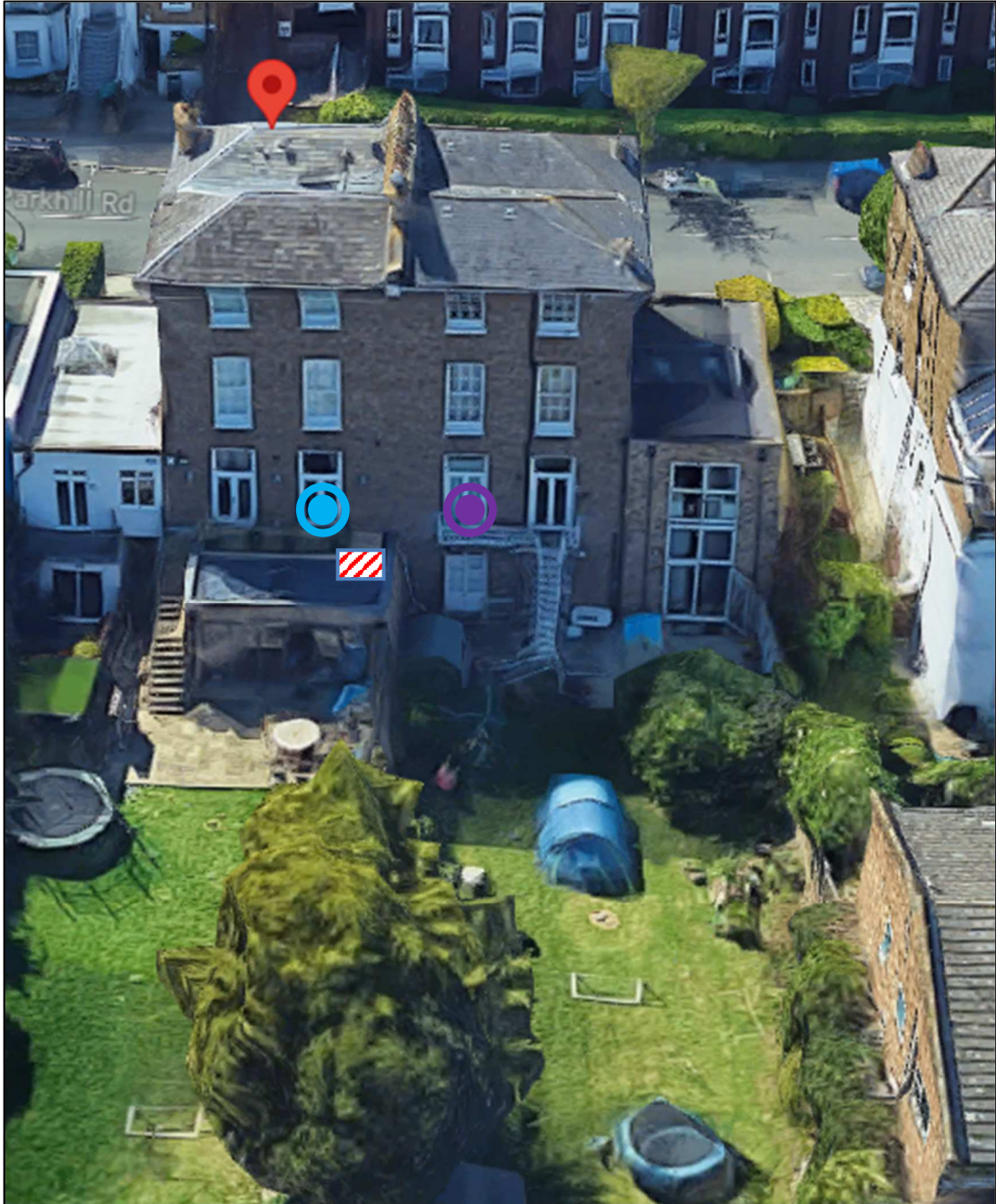
Figure 2.3 Site measurement position, identified receiver and proposed plant unit installation (Image Source: Google Maps)
