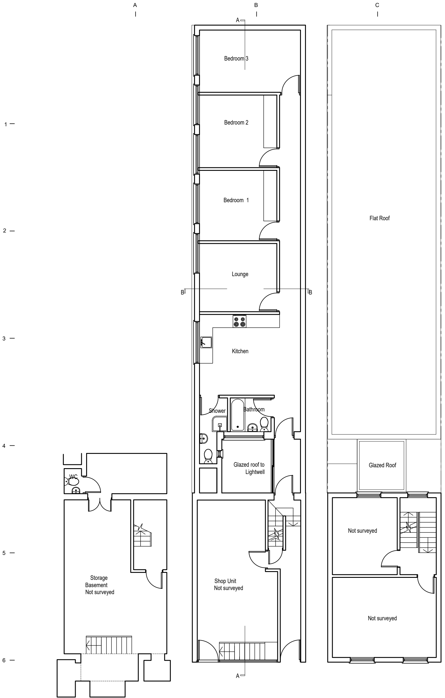
6A EXISTING BASEMENT PLAN SCALE 1:100
